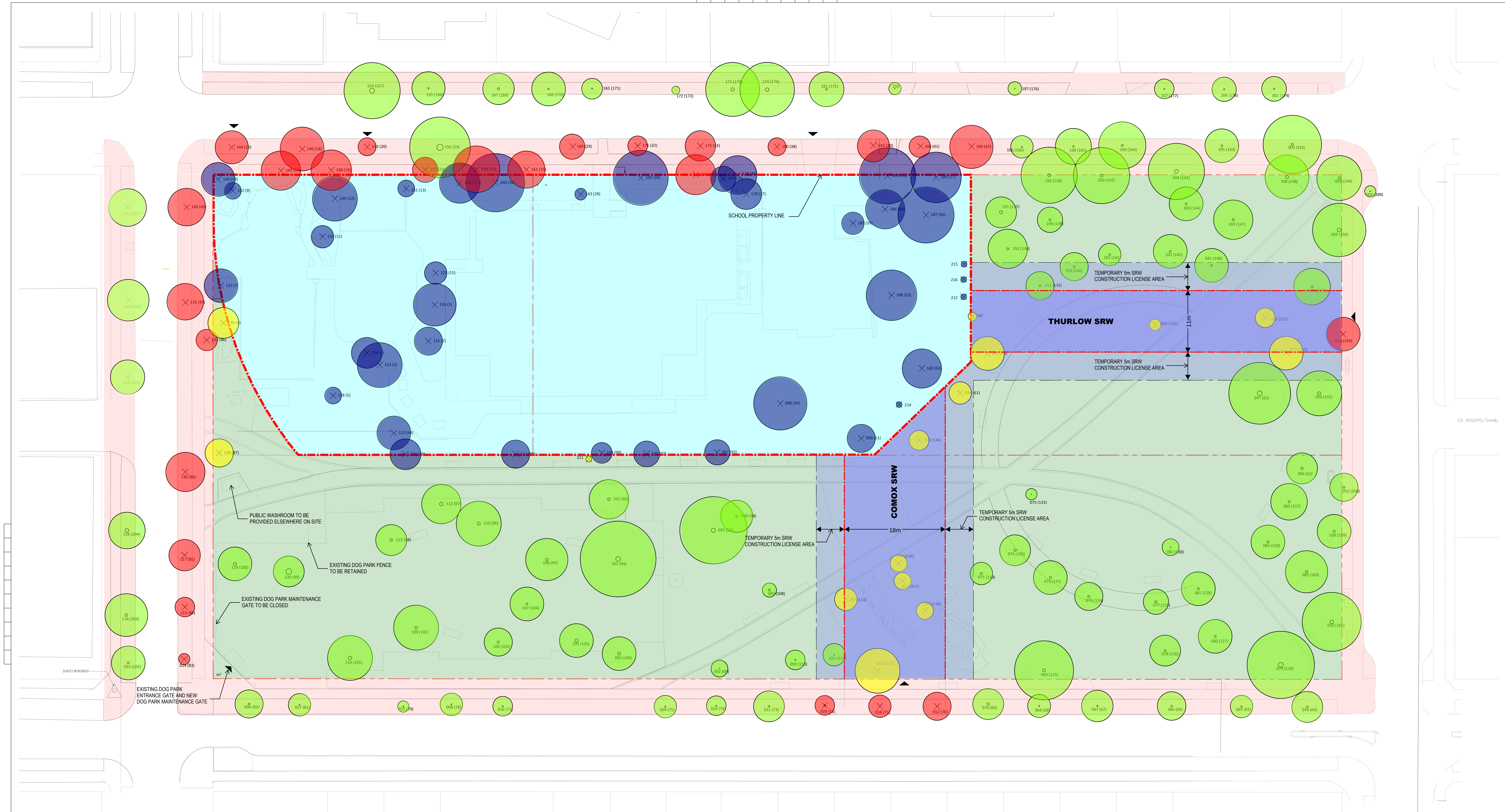
1 TREE MANAGEMENT PLAN SCALE: 1:250
