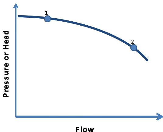
Figure 7: Typical Characteristic Curve for Centrifugal Pump
