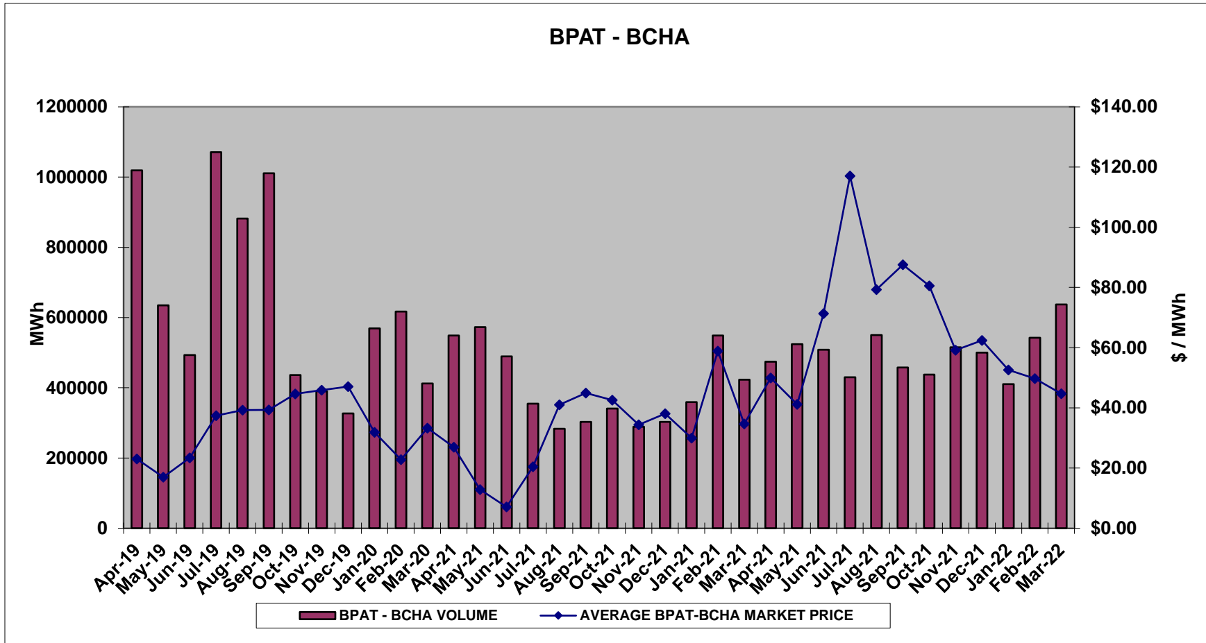
Graph 5: This graph illustrates the relationship between the Network Economy transmission volume and the average Market Price per month from April 2019 to March 2022 for the BPAT–BCHA path.
