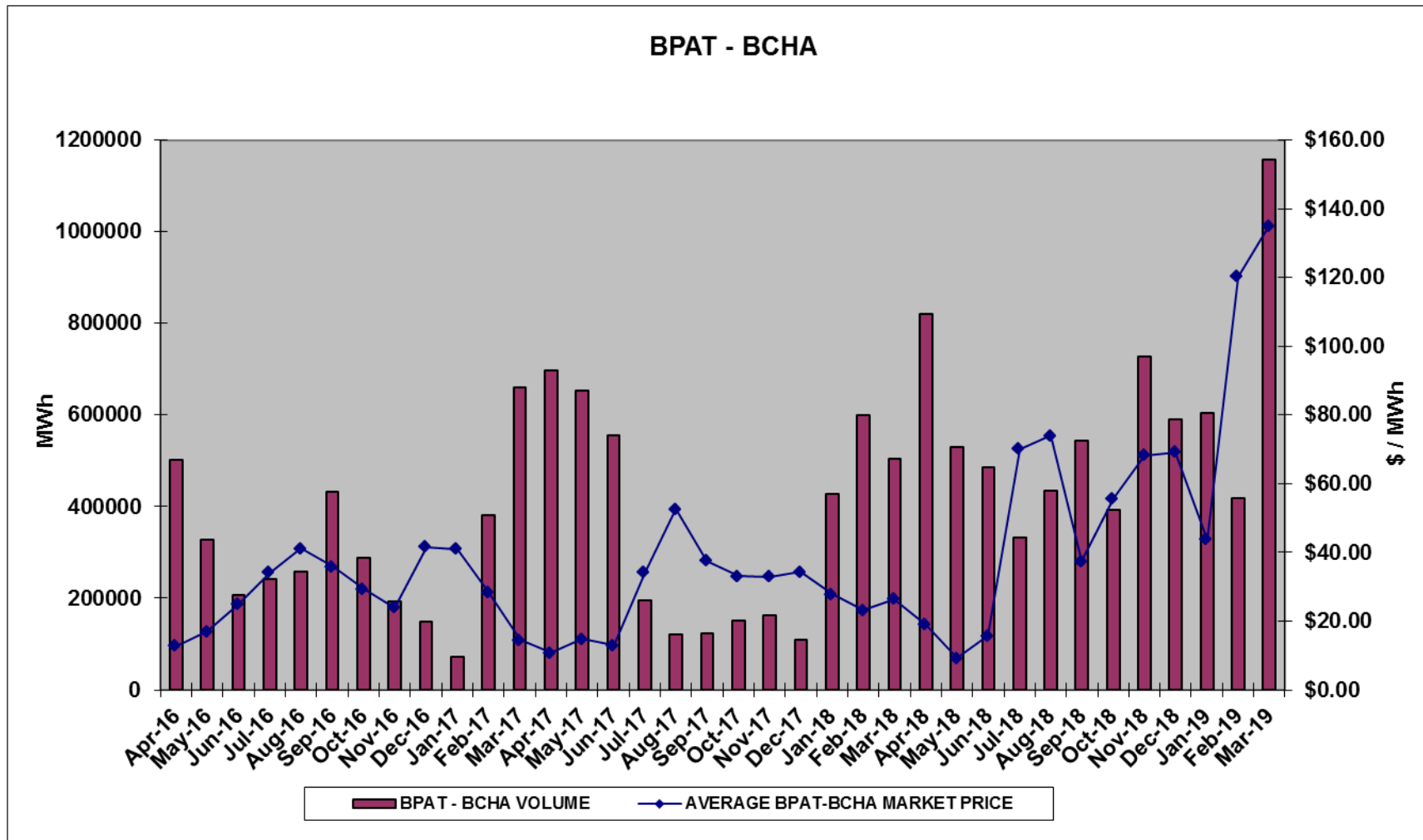
Graph 5: This graph illustrates the relationship between the Network Economy transmission volume and the average Market Price per month from April 2016 to March 2019 for the BPAT–BCHA path.
