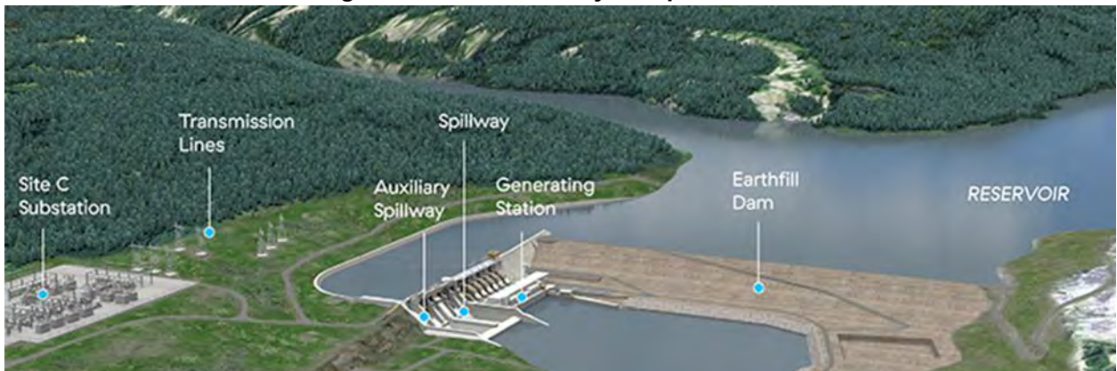
Figure 6-11 Site C Key Components
