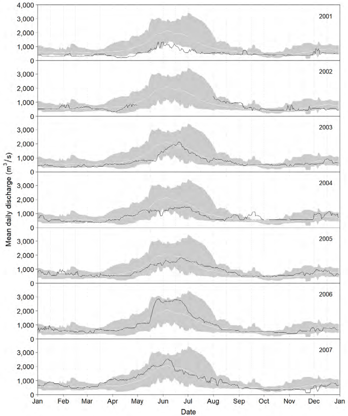
Figure D4. Mean daily discharge ( m^3/s ) for the Kootenay River at Brilliant Dam (BRD), 2001 to 2020 (black line). The shaded area represents minimum and maximum mean daily discharge recorded at BRD during other study years between 2001 and 2020. The white line represents average mean daily discharge over the same time period.
