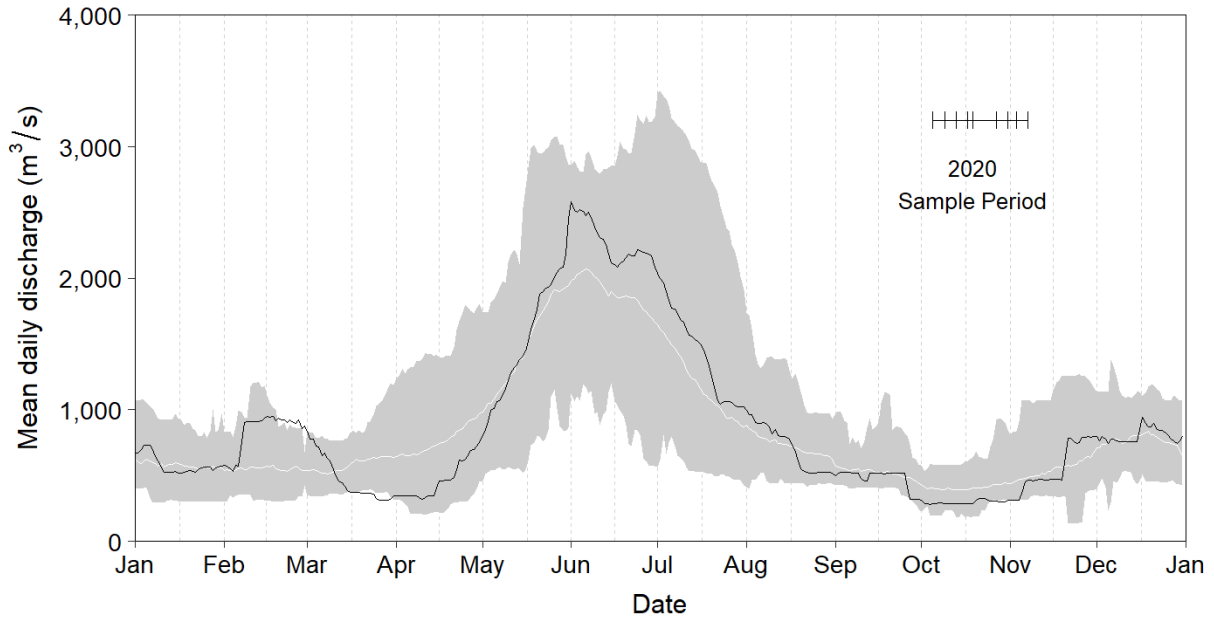
Figure 5: Mean daily discharge (m 3 /s) for the Kootenay River at BRD, 2020 (black line). The shaded area represents minimum and maximum mean daily discharge values recorded at the dam from 2001 to 2019. The white line represents average mean daily discharge values over the same time period.
