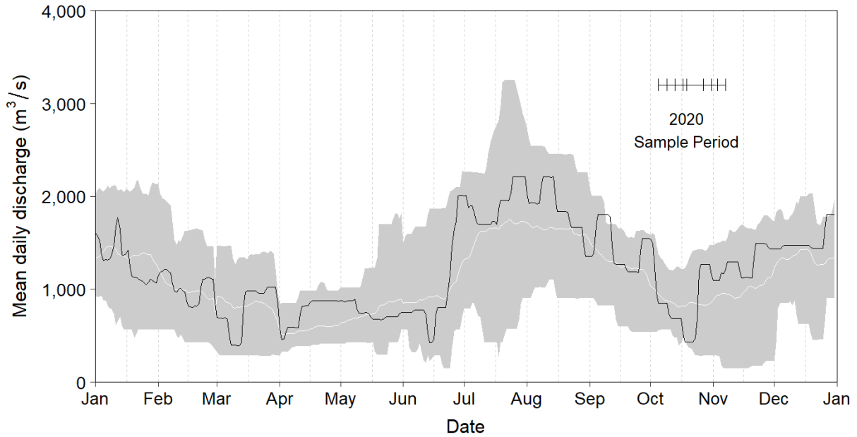
Figure 3: Mean daily discharge (m 3 /s) for the Columbia River at Hugh L. Keenleyside Dam, 2020 (black line). The shaded area represents minimum and maximum mean daily discharge values recorded at the dam from 2001 to 2019. The white line represents average mean daily discharge values over the same time period.
