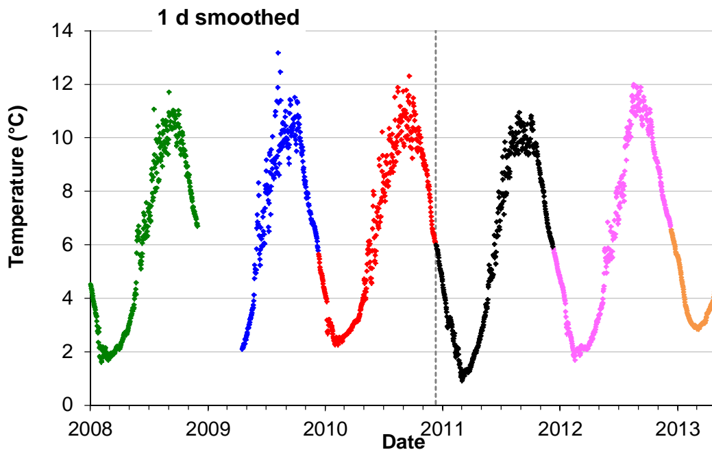
Figure 9. Daily average water temperatures at ‘Station 2’ (below Revelstoke Dam) by date, January 2008 to April 2013. Dotted vertical line at 10 Dec 2010 shows the time at which Unit 5 became operational. Colours correspond to consecutive years, changing on 10 Dec of each year.
