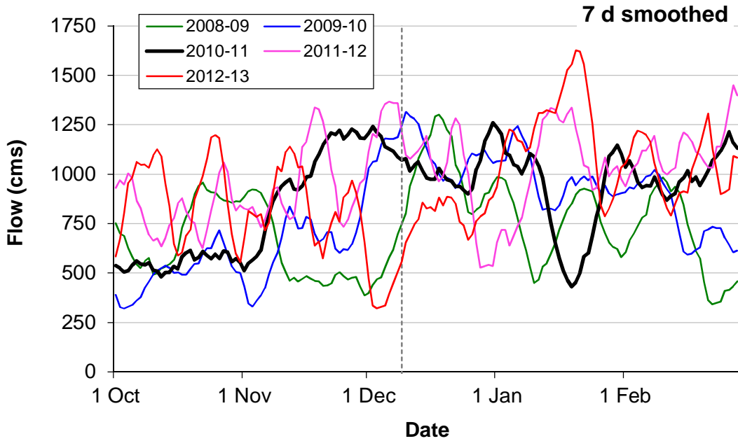
Figure 7. 7-day smoothed Revelstoke Dam turbine + spillway flow by date, October 1 to February 28 shown separately for each winter of data. Dotted vertical line at December 10 shows the time at which Unit 5 became operational in the 2010-2011 winter.
