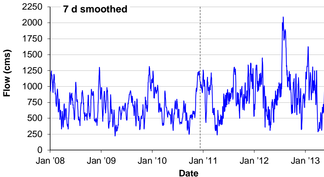
Figure 6. 7-day smoothed Revelstoke Dam turbine + spillway flow by date, January 2008 to April 2013. Dotted vertical line at Dec 10, 2010, shows the time at which Unit 5 became operational.
