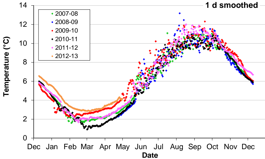
Figure 10. Daily average water temperatures at ‘Station 2’ (below Revelstoke Dam) by date, shown in a different colour for each 365 day period (10 Dec through 9 Dec). Unit 5 became operational on 10 Dec, 2010. The green, blue and red dots predate Unit 5 activity, (2007-2008, 2008-2009, and 2009-2010, respectively) whereas Unit 5 was operational in 2010-2011 (black), 2011-2012 (pink) and 2012-2013 (orange).
