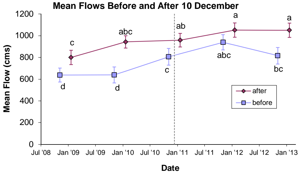
Figure 8. Mean Revelstoke Dam turbine + spillway flow for five winters of data, each split into two time periods: ‘before’: Oct 1 to Dec 10; ‘after’: Dec 11 to Feb 28. Error bars show the 95% confidence intervals around the means. Levels not connected by the same letter are significantly different. Vertical dotted line at December 10, 2010 shows the time at which Unit 5 became operational in the 2010-2011 winter.
