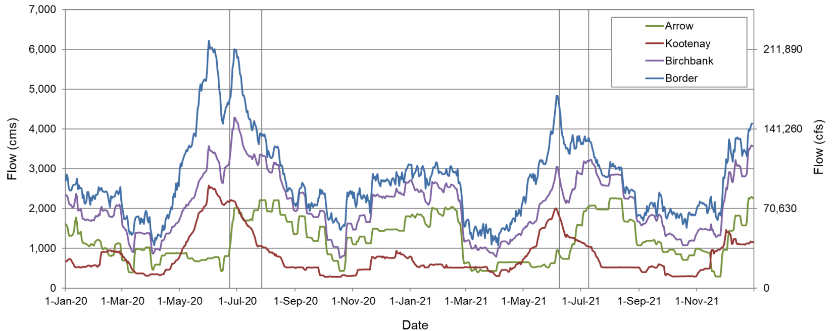
Figure 4a. Mean daily discharge measured from Arrow Reservoir, Kootenay River, Birchbank, and the Canada/U.S. International Border on the lower Columbia River from January 01, 2020 – December 31, 2021. The solid vertical bars represent the first and last estimated spawning date at the Waneta site in 2020 and 2021. No spawning was detected at either Kinnaird or ALH in either year. Estimated spawning dates were based on the developmental stage of collected embryos and/or larvae.
