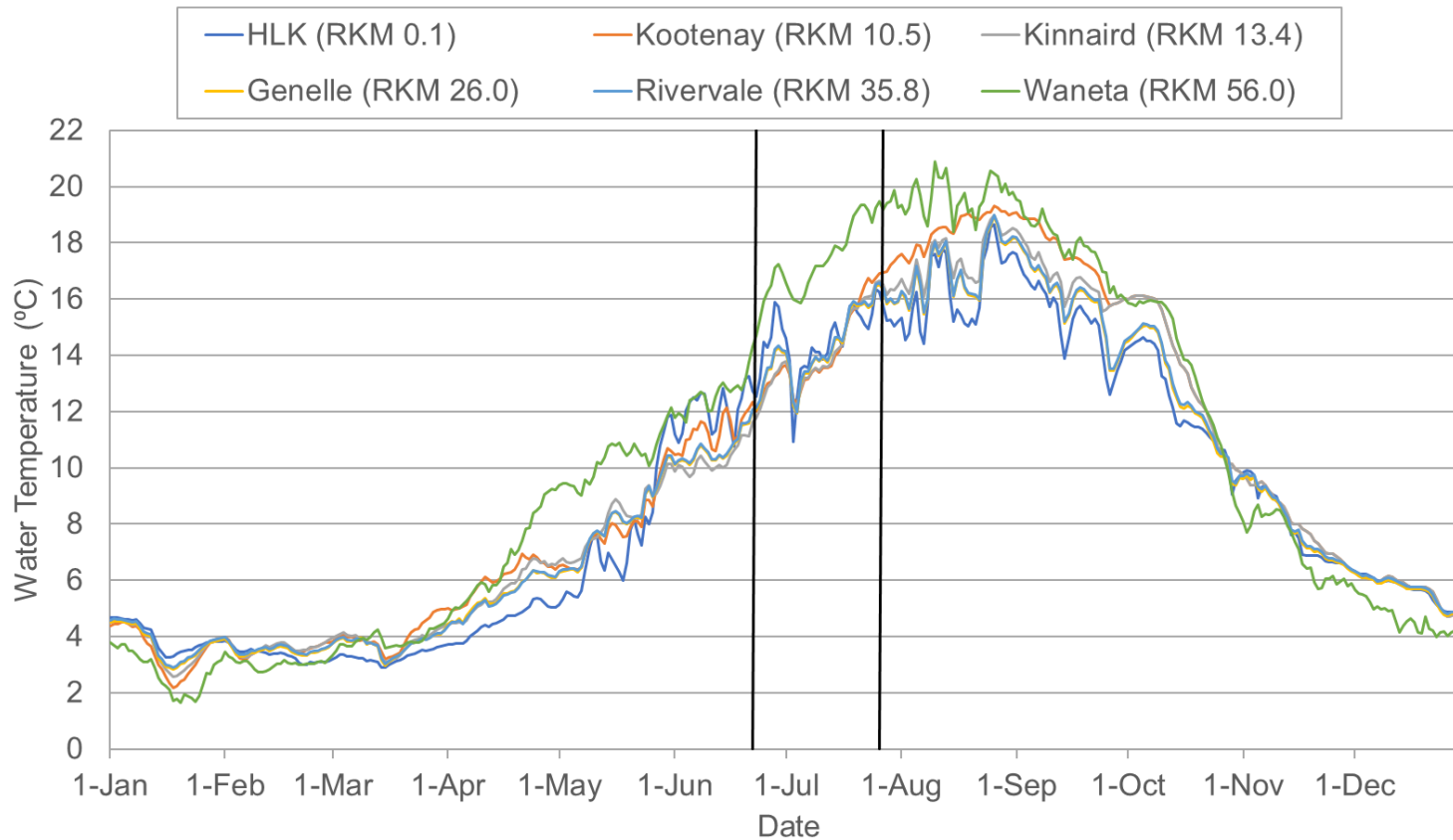
Figure 5a. Mean daily water temperature (°C) of the lower Columbia River in 2020. Data was recorded at locations of Hugh L. Keenleyside dam (HLK; rkm 0.1), Kootenay Eddy (rkm 10.5), Kinnaird (rkm 13.4), Genelle (rkm 26.0), Rivervale (rkm 35.8) and Waneta (rkm 56.0). Missing data is due to lost or damaged temperature loggers. The solid vertical bars represent the first and last estimated spawning date at the Waneta site in 2020. No spawning dates were estimated for Kinnaird and ALH. Estimated spawning dates were based on the developmental stage of collected embryos and/or larvae.
