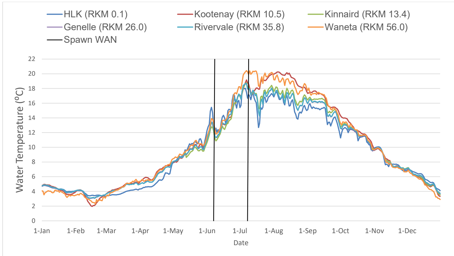
Figure 5b. Mean daily water temperature (°C) of the lower Columbia River in 2021. Data was recorded at locations of Hugh L. Keenleyside dam (HLK; rkm 0.1), Kootenay Eddy (rkm 10.5), Kinnaird (rkm 13.4), Genelle (rkm 26.0), Rivervale (rkm 35.8) and Waneta (rkm 56.0). Missing data is due to lost or damaged temperature loggers. The solid vertical bars represent the first and last estimated spawning date at the Waneta site in 2021. No spawning dates were estimated for Kinnaird and ALH. Estimated spawning dates were based on the developmental stage of collected embryos and/or larvae.
