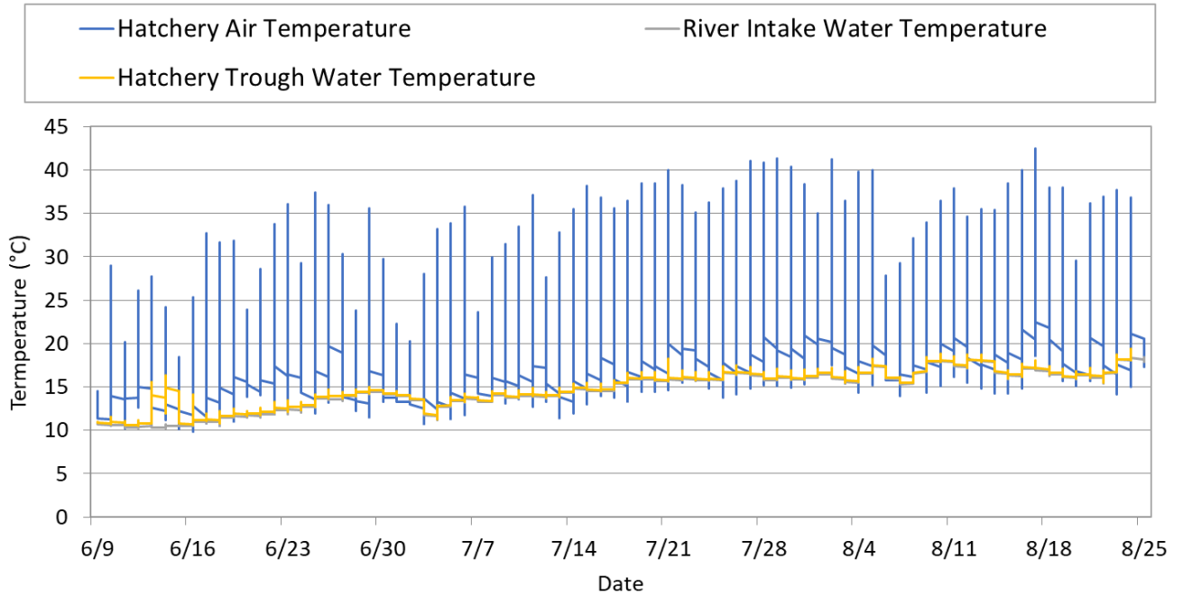
Figure 6a. Hourly temperature (°C) recorded at the lower Columbia River (LCR) Streamside Incubation Facility in 2020. Data includes air temperature inside the facility, and water temperatures of the LCR and incubation tanks.
