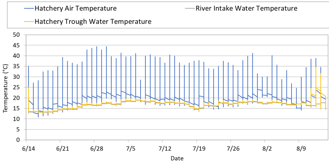
Figure 6b. Hourly temperature (°C) recorded at the lower Columbia River (LCR) Streamside Incubation Facility in 2021. Data includes air temperature inside the facility, and water temperatures of the LCR and incubation tanks.
