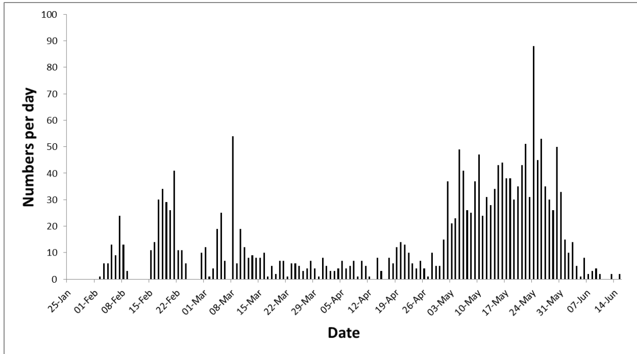
Figure 5.8 Daily catches of juvenile Coho at the RST3 trapping site in reach 3 in the Coquitlam River in 2014. RST3 commenced operation early February, two months prior to full trap deployment, to monitor early season fish movement.
