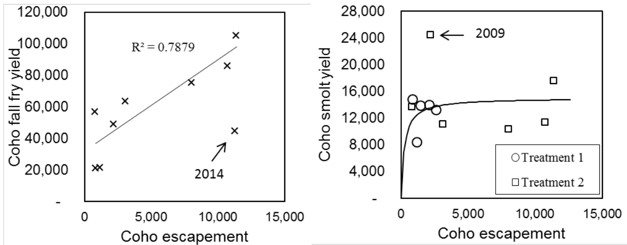
Figure 6.1 Preliminary linear stock-recruitment relationship between Coho escapement and fall fry yield (2006-2014) and Beverton-Holt stock-recruitment relationship between Coho escapement (upstream of RST2) and total smolt yield in the Coquitlam River during Treatment 1 (2004-2008 smolt years), and during the first 6 years of Treatment 2 (2009-2014 smolt years).
