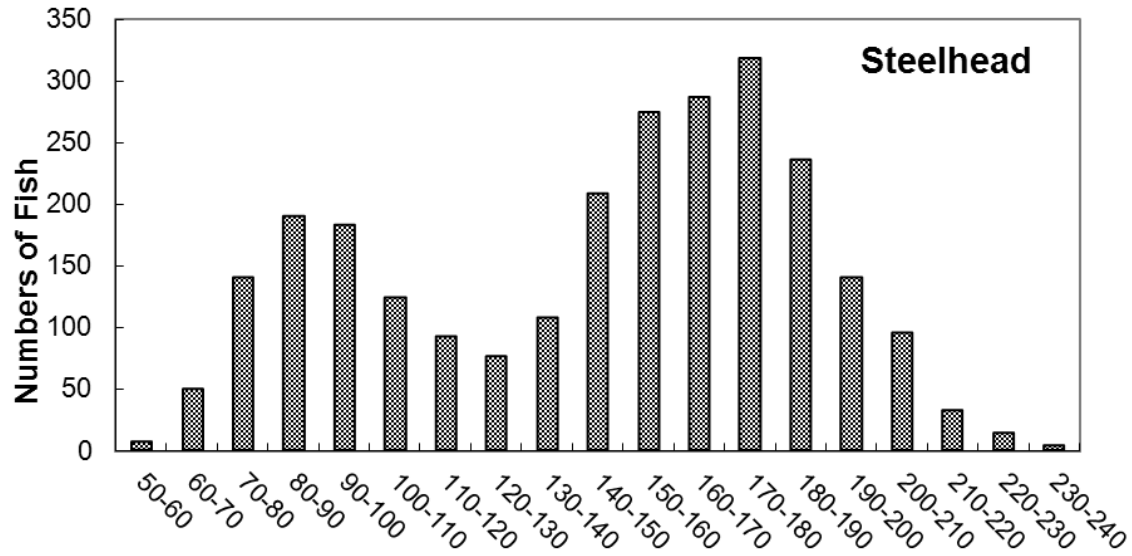
Figure 5.6 Length-frequency histogram for Steelhead captured in the Coquitlam River in 2014 (data pooled for all trap sites).
