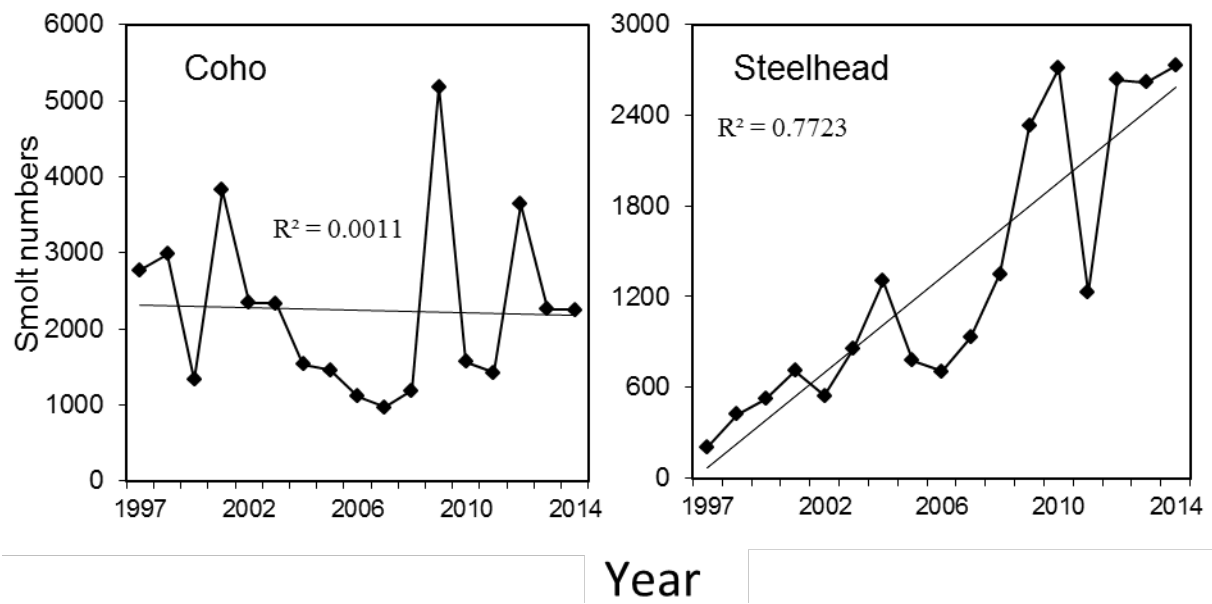
Figure 6.3 Annual numbers of Coho and Steelhead smolts in reach 4 of Coquitlam River during 1997-2014.
