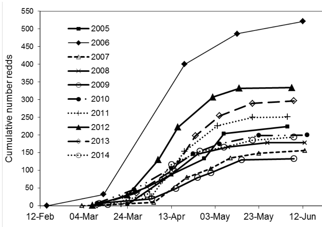
Figure 3.4 Cumulative proportion of the total Steelhead redd count observed over time during 2005 -2014.
