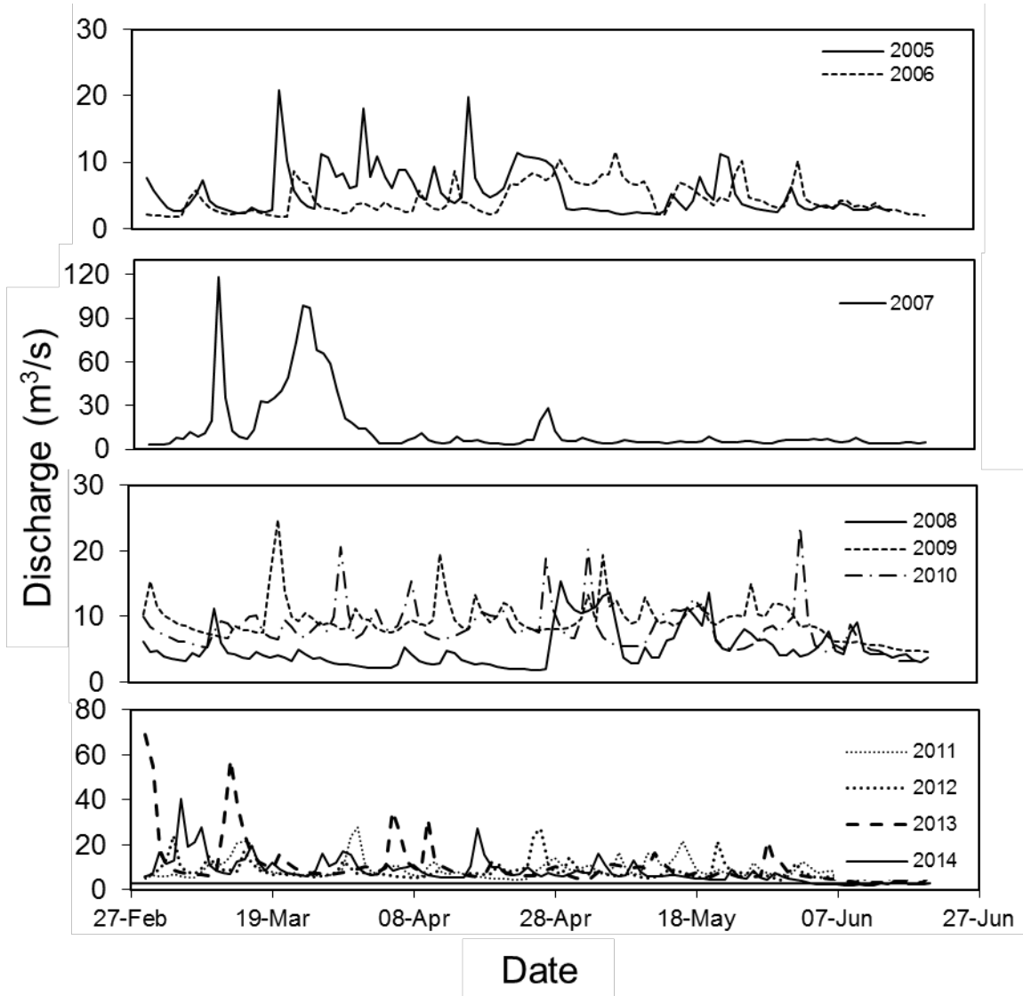
Figure 3.3 Discharge (cms) in Coquitlam River at Port Coquitlam during Steelhead spawning period in 2005 - 2014 (Water Survey of Canada station 08MH002).
