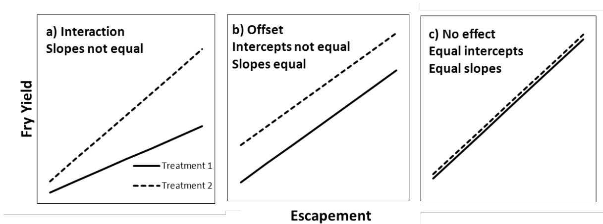
Figure 6.7 Three possible outcomes of the comparisons of fry per spawner stock-recruitment relationships during Treatments 1 and 2, assuming no density dependent interactions. The interaction (a) and offset (b) are examples of how flow treatments could affect fry production either individually or in combination.
