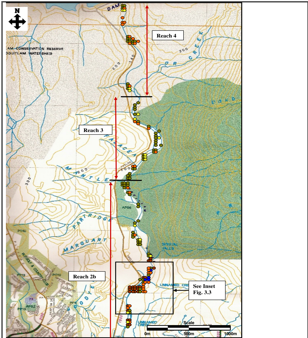
Figure 3.1 Steelhead redd locations in reaches 2b-4 in Coquitlam River in 2006, which was the highest escapement year during 2005-2013. Coquitlam Dam is the upstream boundary of the survey area. See Figure 3.2 for redd symbol legend.
