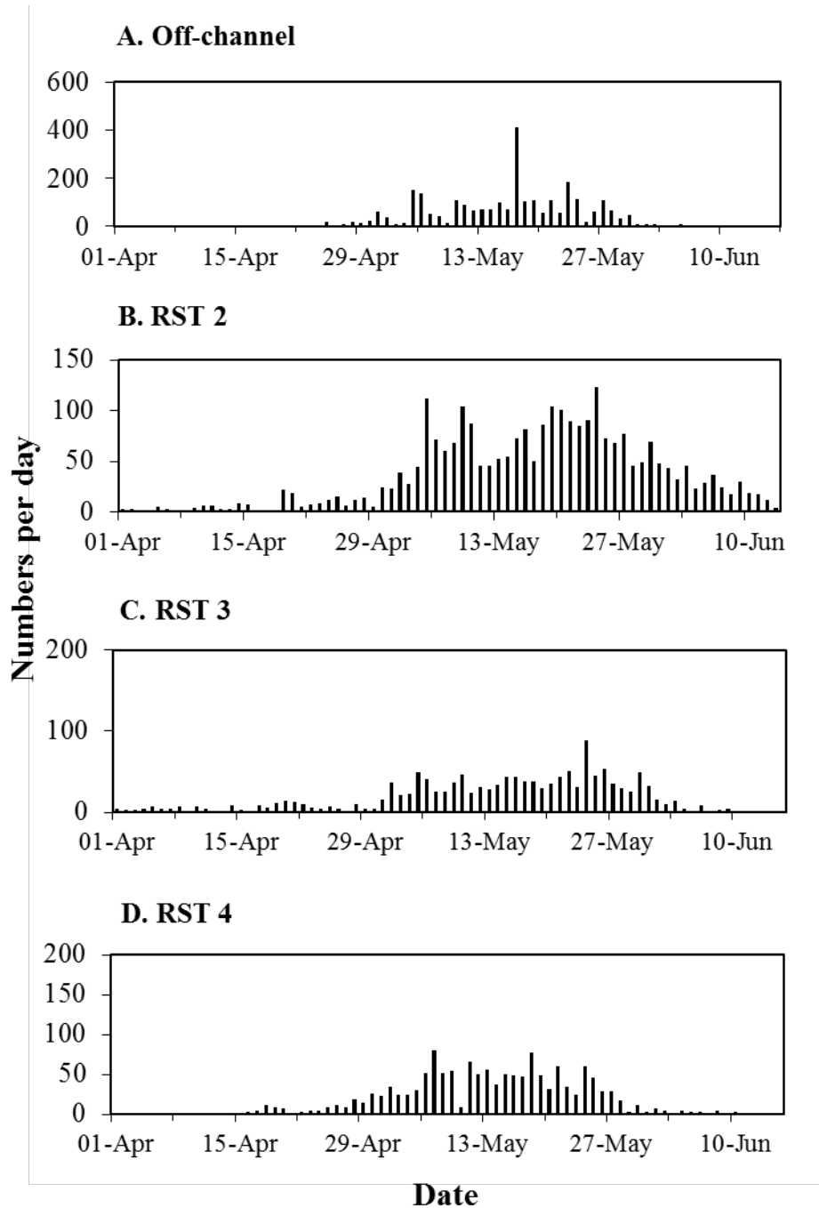
Figure 5.3 Daily catches of Coho smolts at downstream weirs in three off-channel sites (pooled data) and at three rotary screw trapping locations in the Coquitlam River mainstem in 2014. See Table 5.1 for start and end dates for individual trapping sites.
