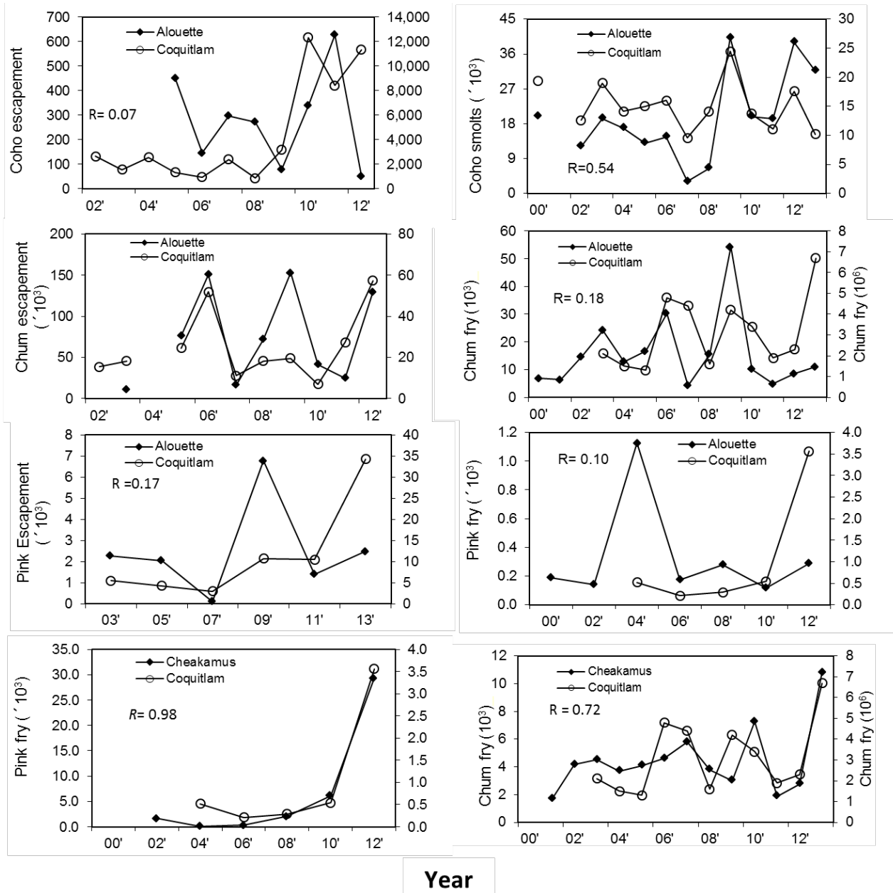
Figure 6.2 Scatterplots of escapement and smolt yield in the Coquitlam River versus that in the Cheakamus and Alouette rivers during 2000-2014. Values for the Coquitlam River are given on the right-hand axis, and values for other streams are given on the left-hand axis.
