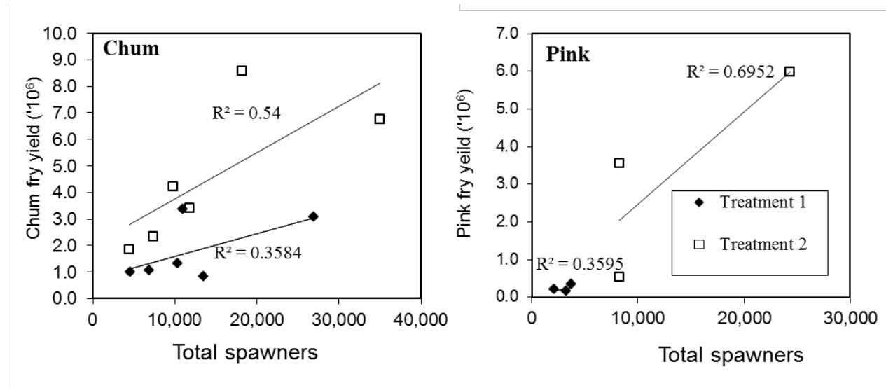
Figure 6.6 Preliminary stock-recruitment relationships for outmigrating Chum and Pink smolts (2002-2014) versus brood escapements in the Coquitlam River.
