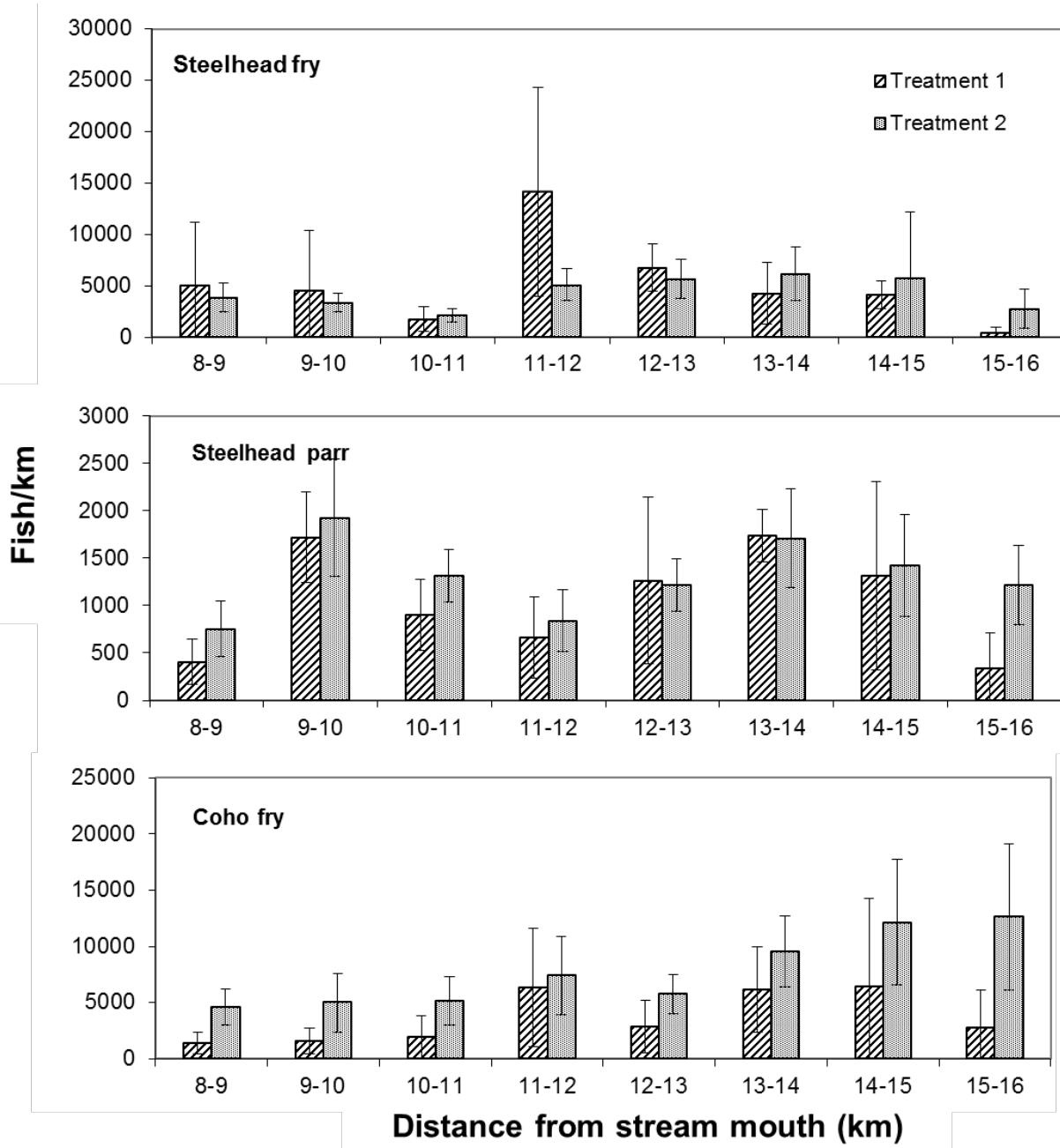
Figure 4.3 Linear distribution of juvenile salmonids in the Coquitlam River during Treatment 1(2006-2008) and Treatment 2 (2009-2014). Bars represent mean abundance estimates and 95% confidence intervals for years under flow Treatments 1 and 2. Estimates are based on calibrated snorkeling counts at 10-12 sampling sites 2006-2013 and 24 sites in 2014.
