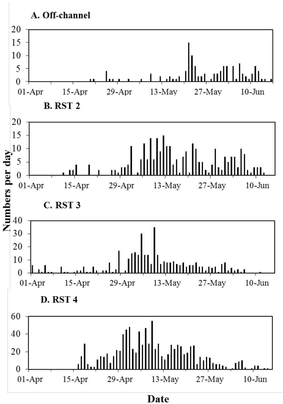
Figure 5.4 Daily catches of Steelhead smolts at downstream weirs in three off-channel sites (pooled data) and at three rotary screw trapping locations in the Coquitlam River mainstem in 2014. See Table 5.1 for start and end dates for individual trapping sites.
