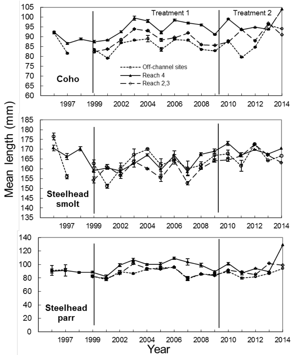
Figure 6.4 Mean annual forklengths for Coho smolts and Steelhead smolts (age 2+ and 3+ combined) and parr in different habitats in the Coquitlam River, 1996-2014. Error bars represent \pm 1 standard error.
