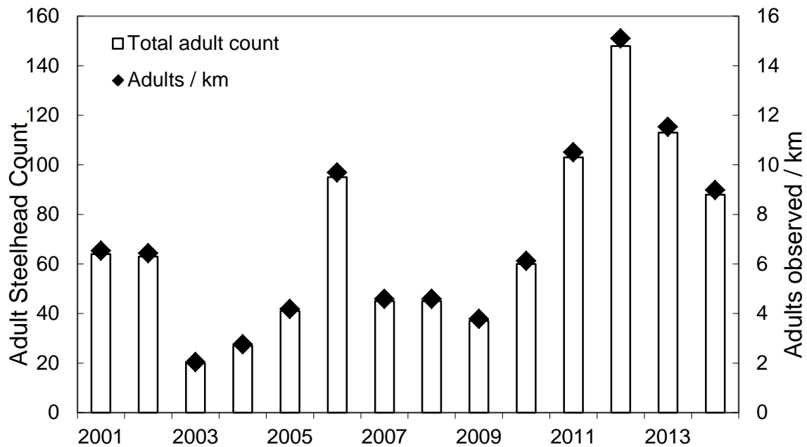
Figure 3.5 Peak counts and densities (fish/km) of adult Steelhead during snorkeling surveys in 2001-2014 (only data for complete surveys of the study area are shown). Data for 2001-2004 were collected as part of a separate study (BCCF, Lower Mainland Branch, data on file).
