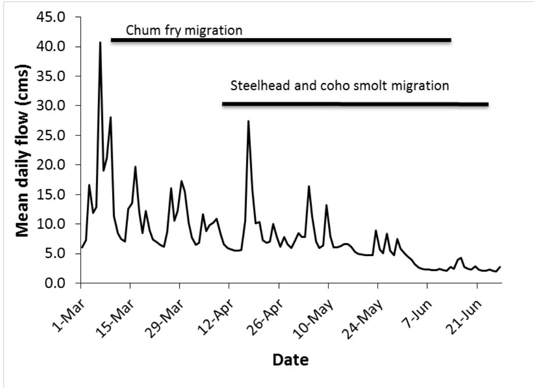
Figure 5.2 Mean daily flows in Coquitlam River at Port Coquitlam during the smolt trapping period in 2014. (Water Survey of Canada, stn. 08MH141). Approximate start times of Chum fry and Steelhead and Coho smolt migration based on captures at all trapping locations during 2014.
