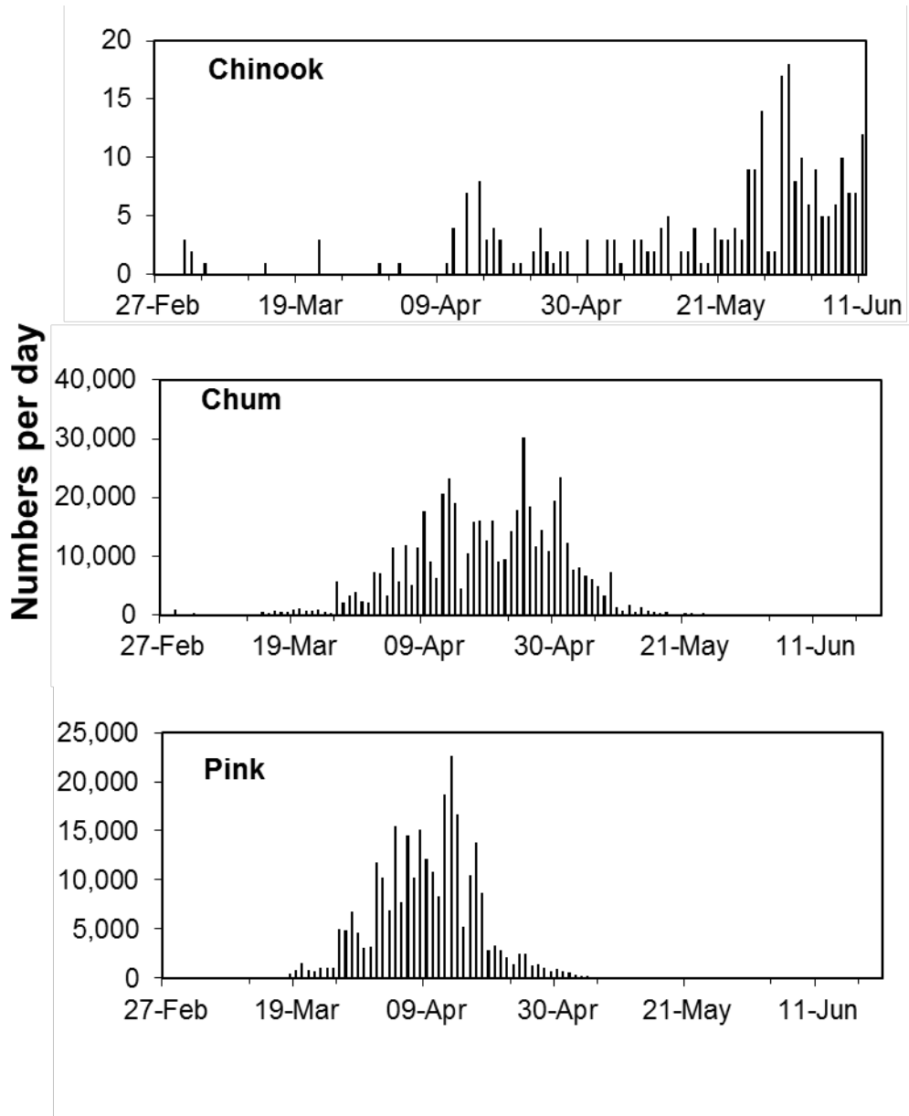
Figure 5.7 Daily catches of Chum and Pink fry at the RST2 trapping site in reach 2, and Chinook smolts at RST2, RST3 and RST4 in the Coquitlam River in 2014. See Table 5.1 for start and end dates of downstream trapping.
