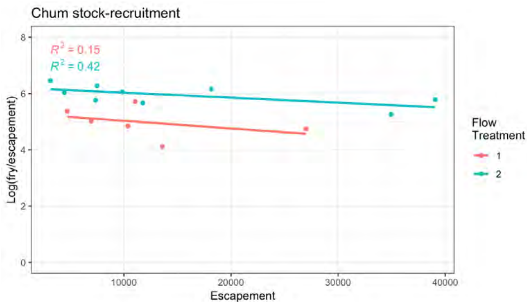
Figure 6.18 Adult-to- \ln(\text{fry}/\text{adult}) stock-recruitment relationships of Chum during flow Treatment 1 (red 2002-2008) and Treatment 2 (teal 2009-2016) from 7.5 km of the Coquitlam River used for the ANCOVA tests as to whether flow treatment had a significant effect of productivity.
