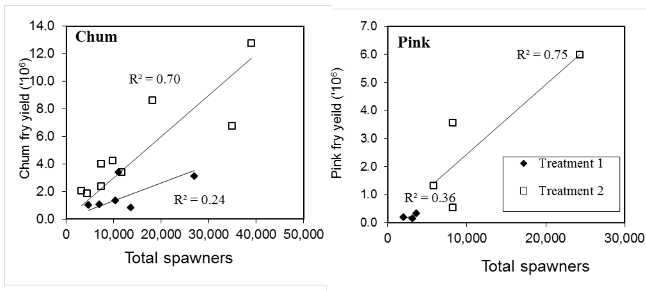
Figure 6.17 Preliminary escapement-to-fry stock-recruitment relationships of Chum and Pink Salmon during flow Treatment 1 (2002-2008) and Treatment 2 (2009-2017) from 7.5 km of the Coquitlam River. The best-fit lines intercept the x and y axis at 0 as is typical of stock-recruitment relationships. Note that because Pink Salmon spawn every other year in the lower Fraser River watershed, the number of datapoints is half as for Chum. R^2 values reflect the fit of stock-recruitment.
