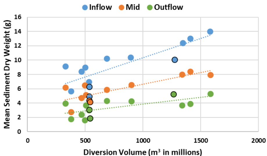
Figure 3.8 Sediment accumulation in each longitudinal zone (i.e., inflow, mid, and outflow) of Seton Lake according to diversion volume from Carpenter Reservoir based on Years 4 to 8 (2016–2020) results. Points with black border represent 2020 data; Plain points are data from previous years. Linear regressions are shown (see Table 3.4 for regression parameters).
