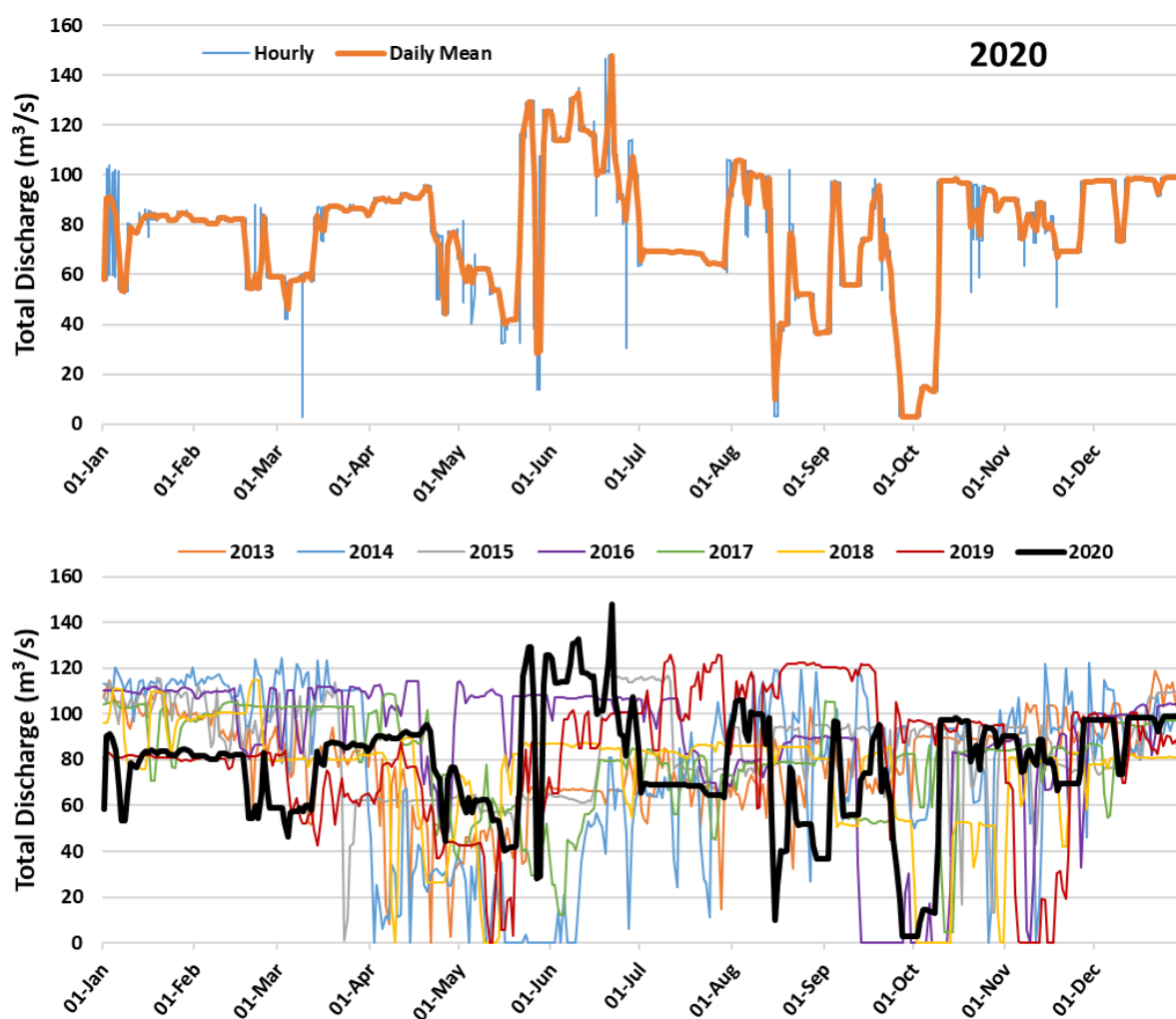
Figure 3.1 Total Discharges from the Bridge 1 and Bridge 2 Generating Stations into Seton Lake from January to December. Hourly and daily means for Year 8 (2020) are shown in the upper plot, and daily means for each monitoring year (2013 - 2020) are in the lower plot.
