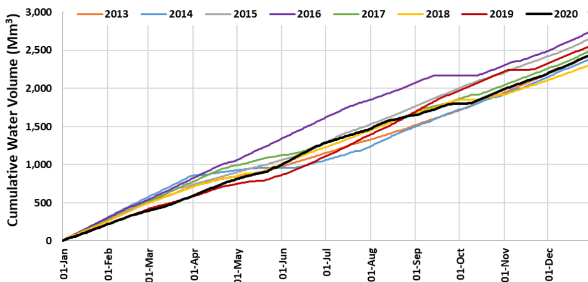
Figure 3.2 The daily cumulative inflow volume from the Bridge 1 and 2 Generating Stations, 2013 to 2020 (Monitoring Years 1 to 8).
