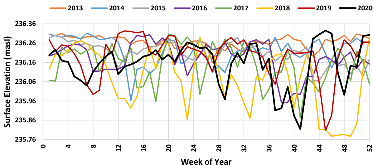
Figure 3.3 Mean weekly surface elevations of Seton Lake recorded in the forebay of Seton Dam across the year, 2013 to 2020. Note: the y-axis range spans the licensed operating range referenced in the Water Use Plan (BC Hydro 2011).
