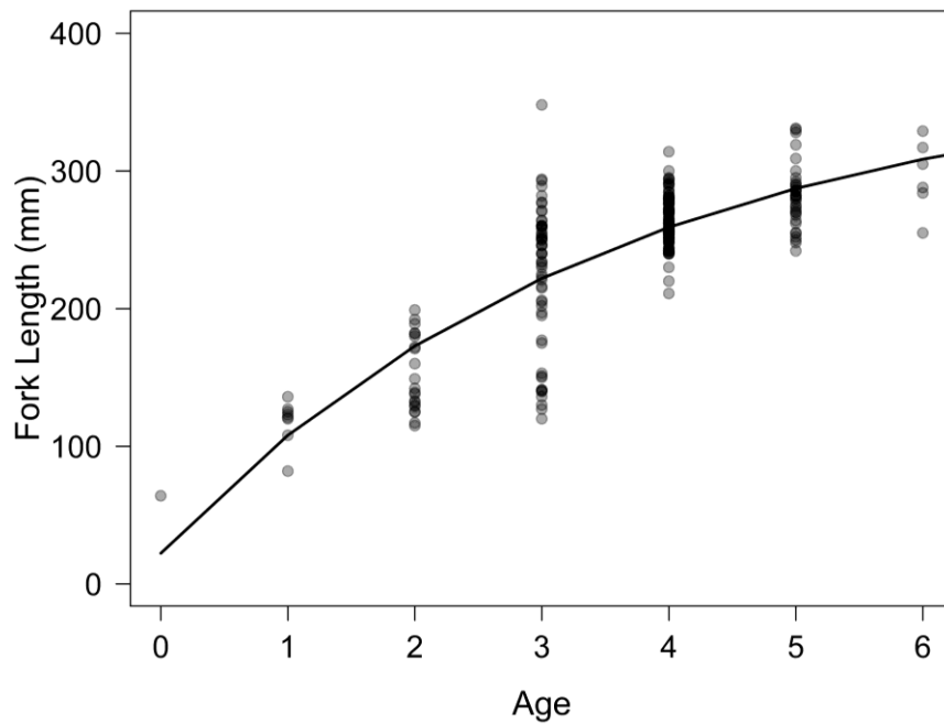
Figure 3.23 Von Bertalanffy growth model for Mountain Whitefish fork length (mm) and observed ages (all study years combined). Transparency shows point overlap.
