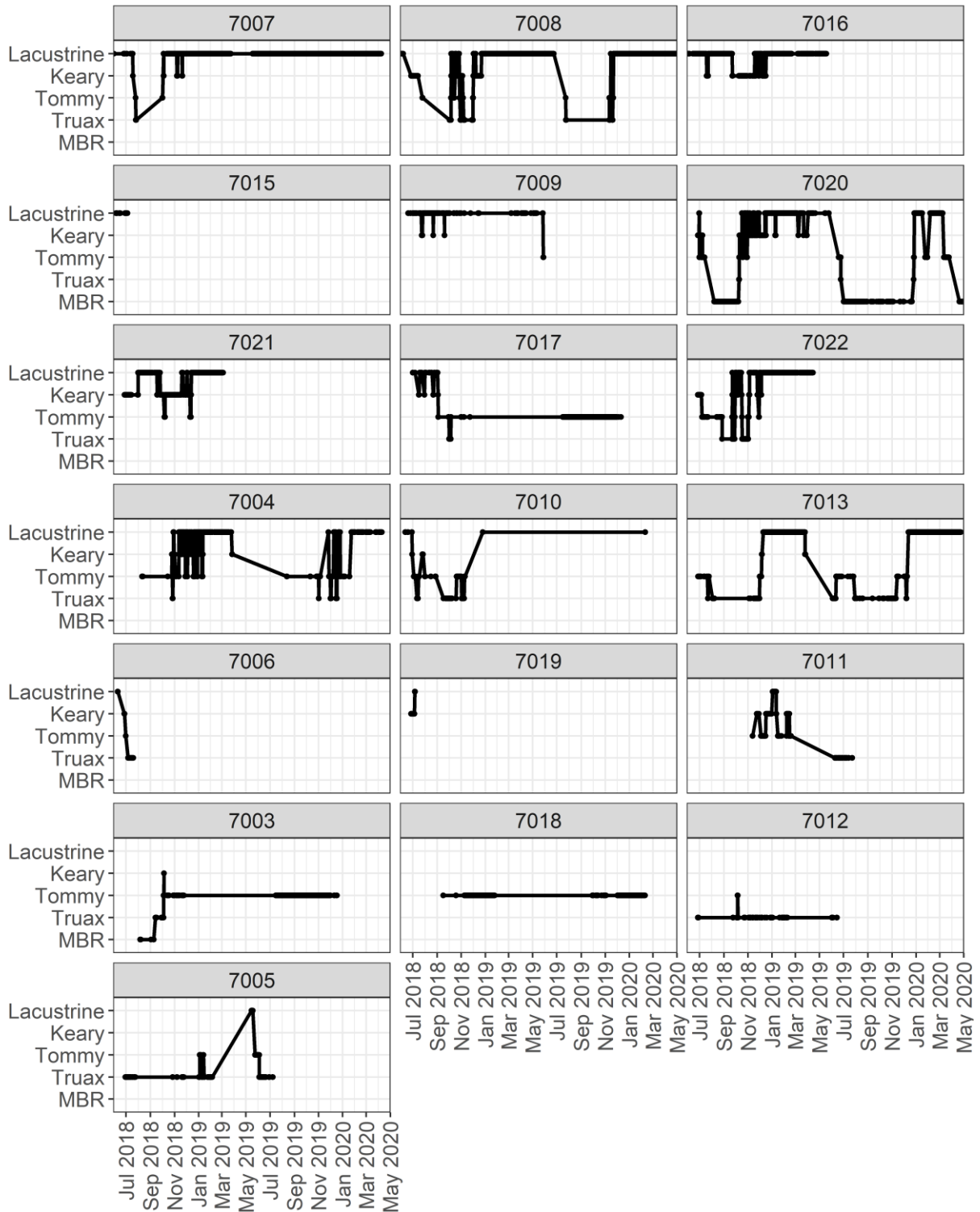
Figure 3.15 Movement summaries for acoustic Bull Trout tagged in May and June of 2018. Points show detections, while connecting lines represent presumed location.
