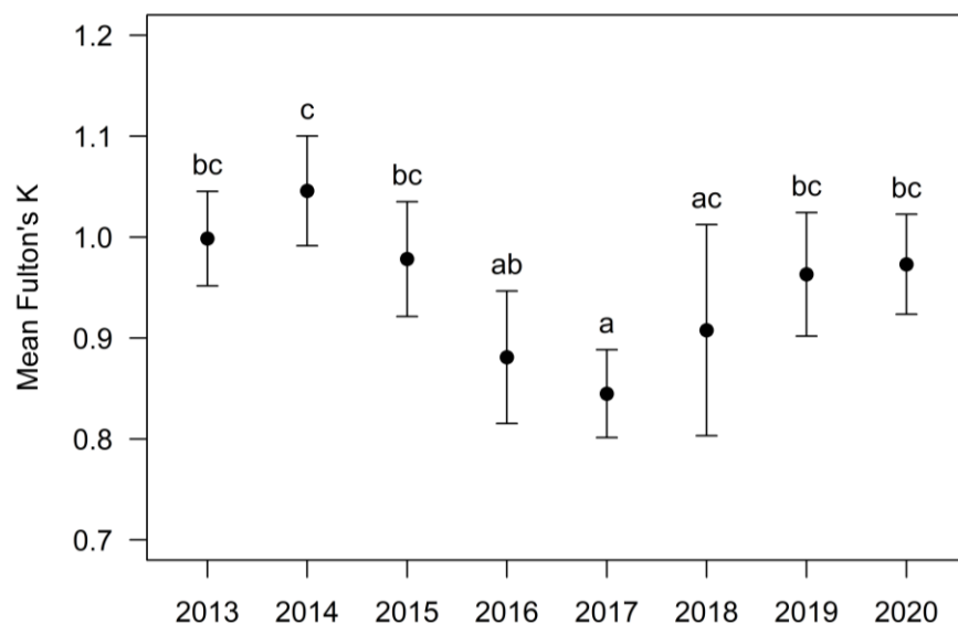
Figure 3.20 Mean annual condition factor (with 95% CI) for Rainbow Trout (Carpenter Reservoir only). Means with the same significance letter are statistically equal.
