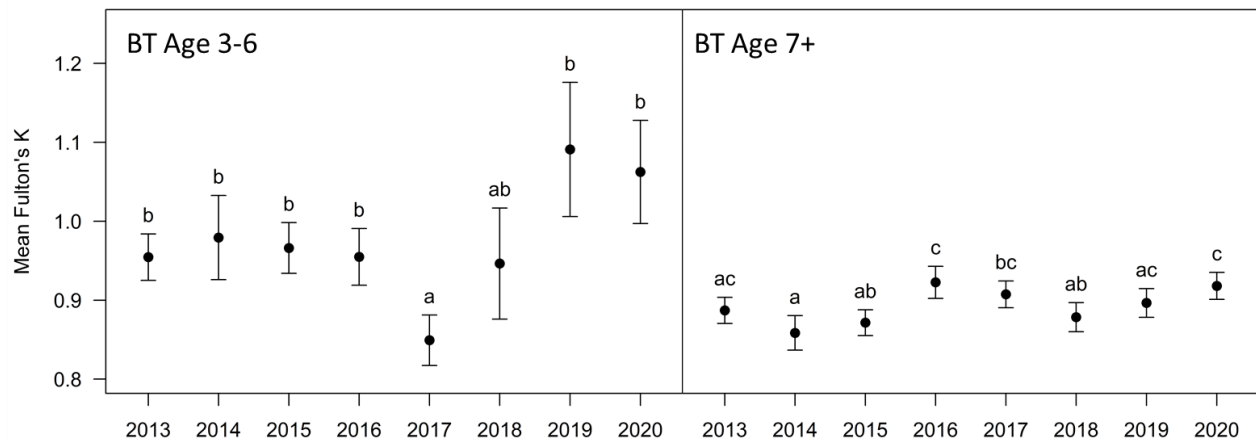
Figure 3.18 Mean annual condition factor (Fulton's K ) and 95% CI for Bull Trout in Carpenter Reservoir. Means with the same significance letter are statistically equal.
