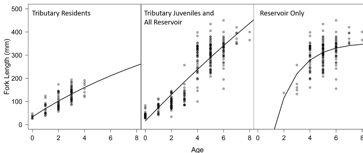
Figure 3.21 Von Bertalanffy growth models for Rainbow Trout fork length (mm) and observed ages separated by life-history type (all study years combined). Transparency shows point overlap.
