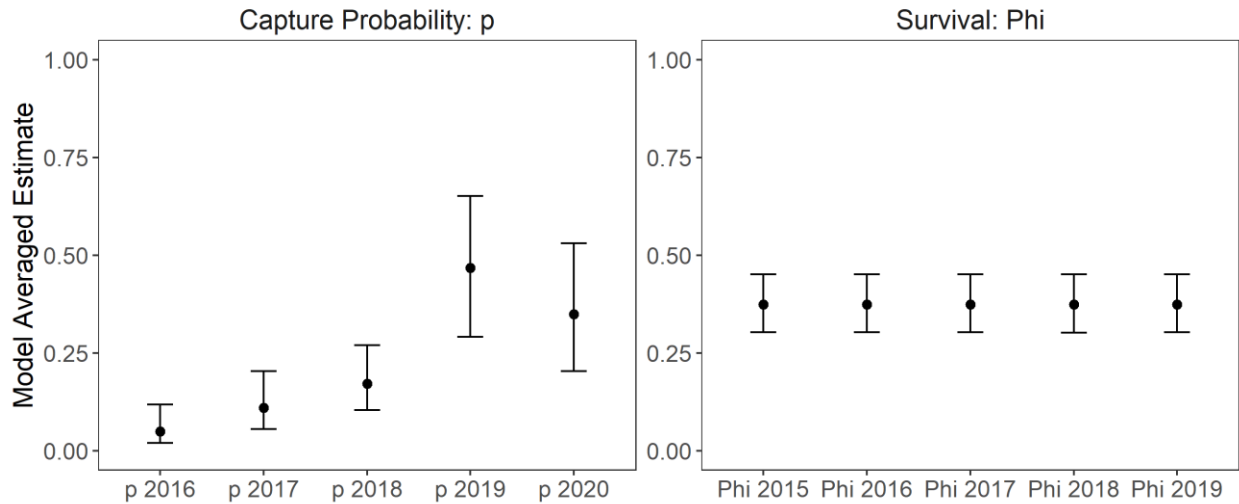
Figure 3.13 Model averaged capture and survival probabilities for the Carpenter Reservoir open mark-recapture model.
