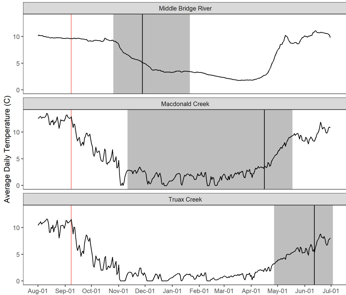
Figure 3.26 Kokanee peak 50% hatch date (black line) and estimated 50% hatch window (shaded grey area) for eggs laid in 2018. Hatching dates were calculated using the peak kokanee migration date (red line) and the maximum and minimum extent of the migration (not shown).
