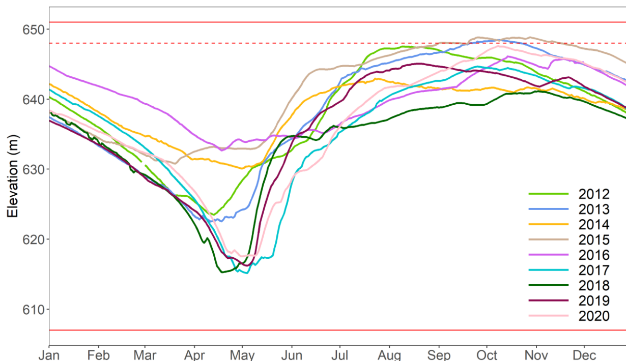
Figure 3.1 Carpenter Reservoir elevations (2012 to 2020). Solid red lines represent maximum and minimum operational targets of 606.55 m and 651.08 m, respectively, and dashed red line represents the soft operational maximum target of 648 m.
