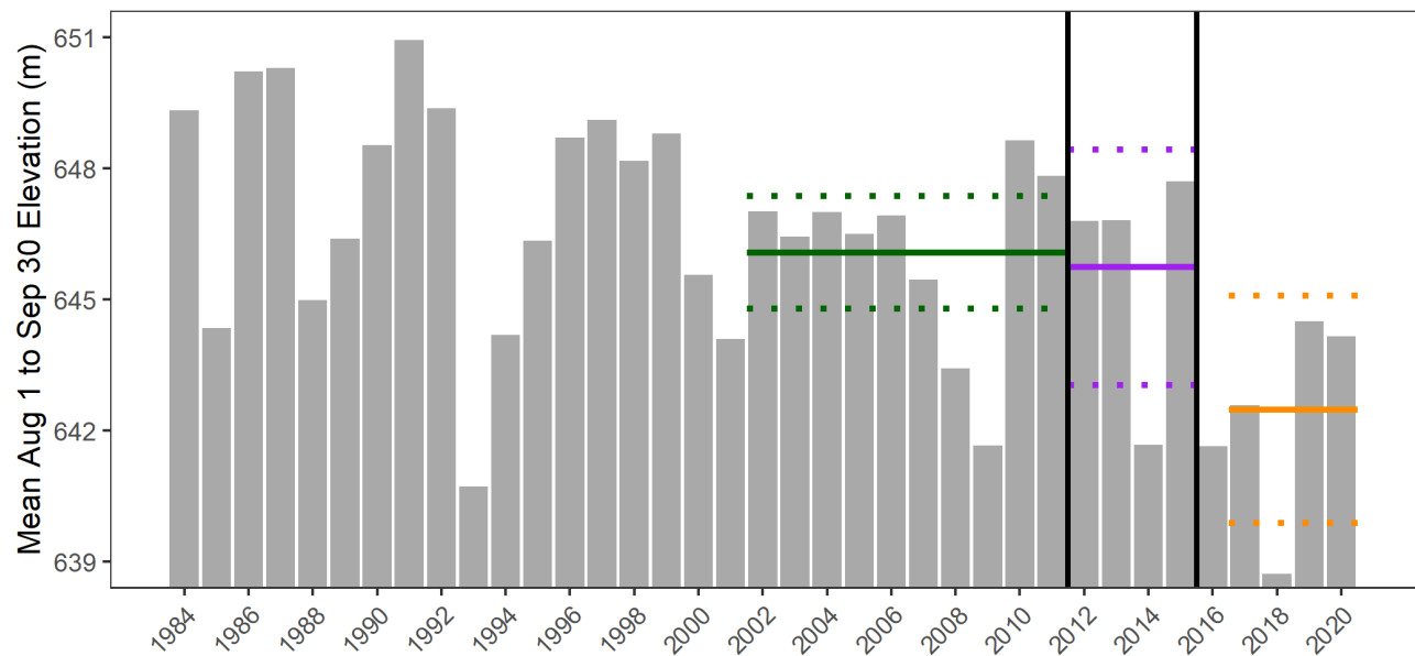
Figure 3.3 Historic average Carpenter Reservoir elevation from August 1 to September 30. Green lines show mean elevation (dashed lines represent 95% confidence intervals) from 2002 to 2011, purple lines show mean elevation from 2012 to 2015, and orange lines show mean elevation from 2017 to 2020 (2016 was not included in either N2-2P or Modified Operations because it was a transitional year).
