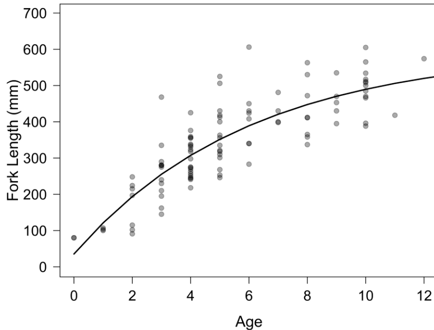
Figure 3.19 Von Bertalanffy growth model for Bull Trout fork length (mm) and observed ages (all study years combined). Transparency shows point overlap.
