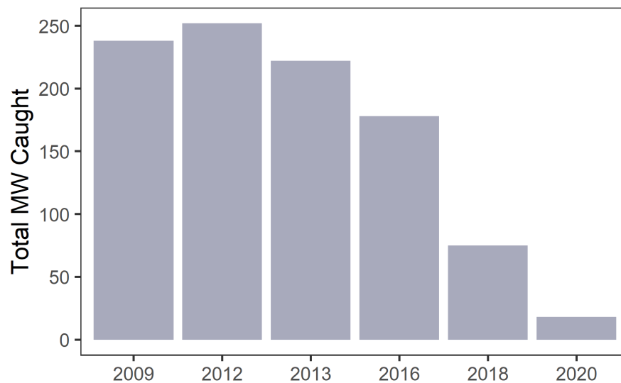
Figure 3.5 Counts of Mountain Whitefish captured during Middle Bridge River spawning assessments from 2009 to 2020. Counts are restricted to between October 25 and December 15 to account for variation in survey duration.
