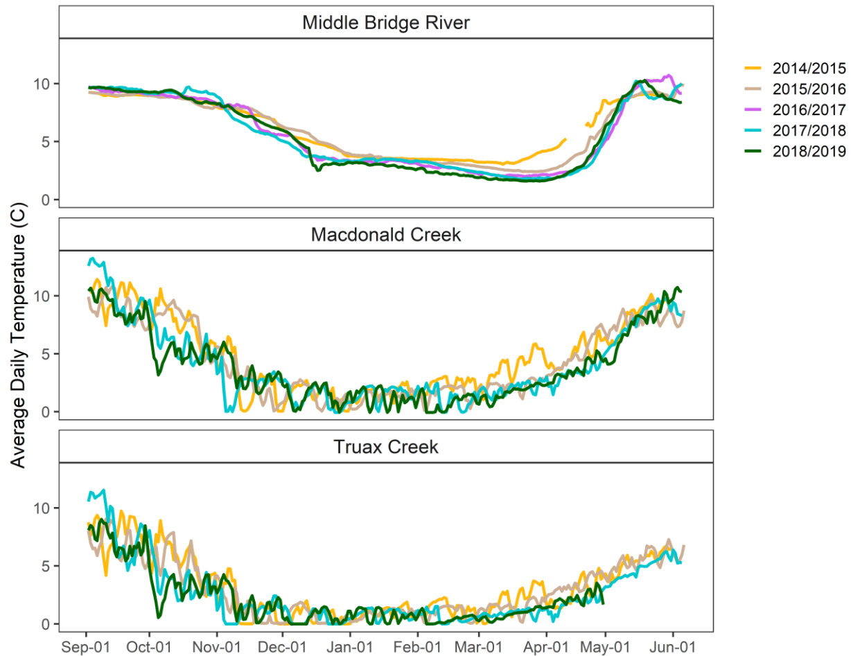
Figure 3.27 Average daily temperatures in Carpenter Reservoir kokanee spawning tributaries during the approximate egg incubation and hatching period from early September to mid-June.
