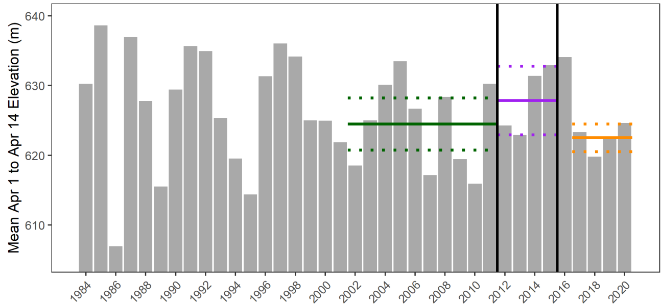
Figure 3.2 Historic average Carpenter Reservoir elevation from April 1 to April 14. Green lines show mean elevation (dashed lines represent 95% confidence intervals) from 2002 to 2011, purple lines show mean elevation from 2012 to 2015, and orange lines show mean elevation from 2017 to 2020 (2016 was not included in either N2-2P or Modified Operations because it was a transitional year).
