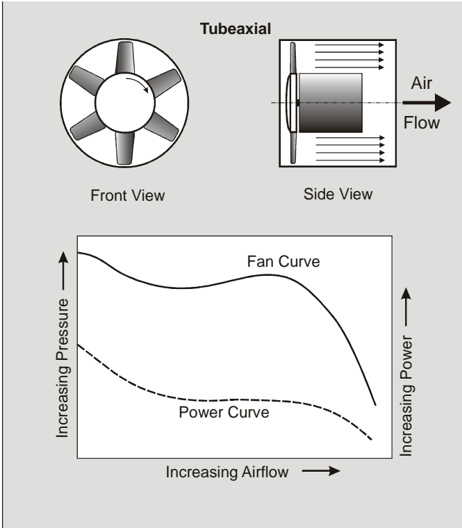
Figure 8: Tubeaxial Fan
