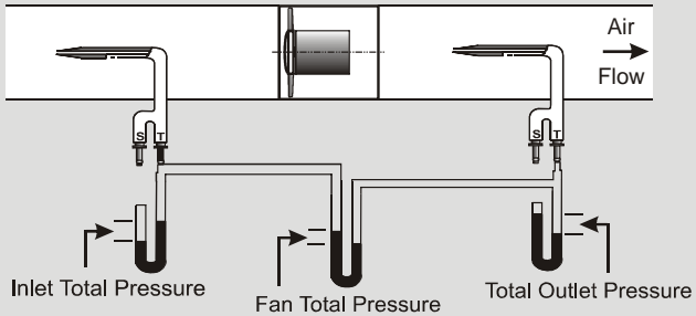
Figure 19: Alternative Methods of Measuring Fan Pressure
