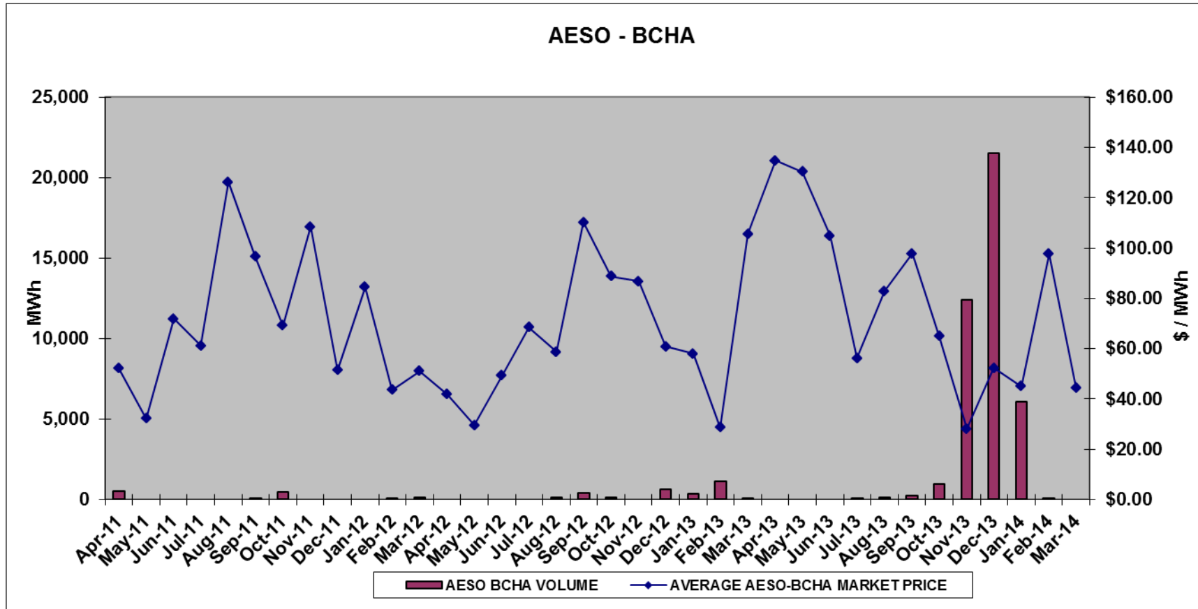
Graph 6: This graph illustrates the relationship between the Network Economy transmission volume and the average Market Price per month from April 2011 to March 2014 for the AESO–BCHA path.
