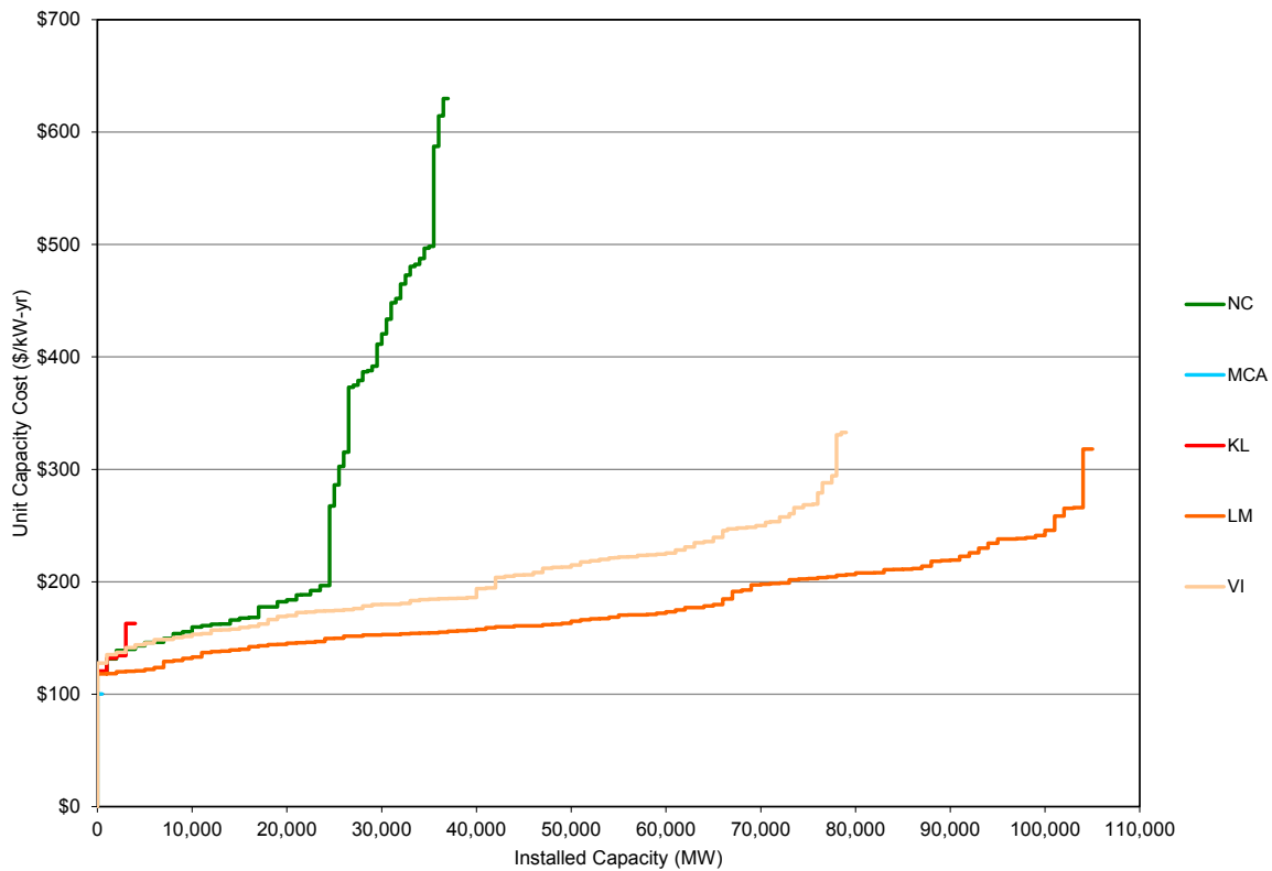
5 Figure 5-13 Pumped Storage POI Supply Curves
