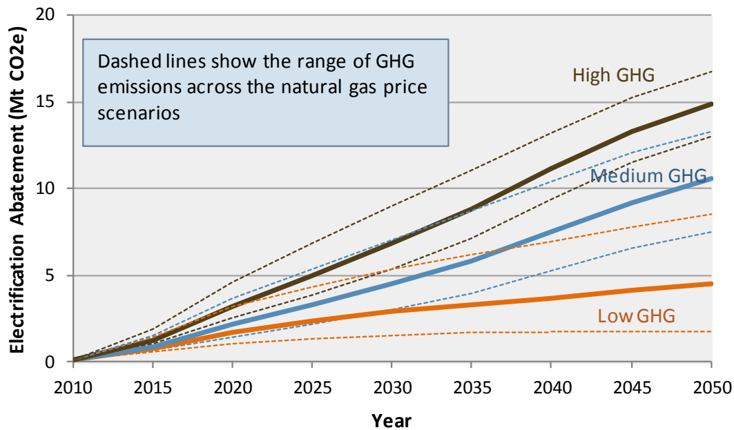
Figure 6: Electrification abatement by scenario
