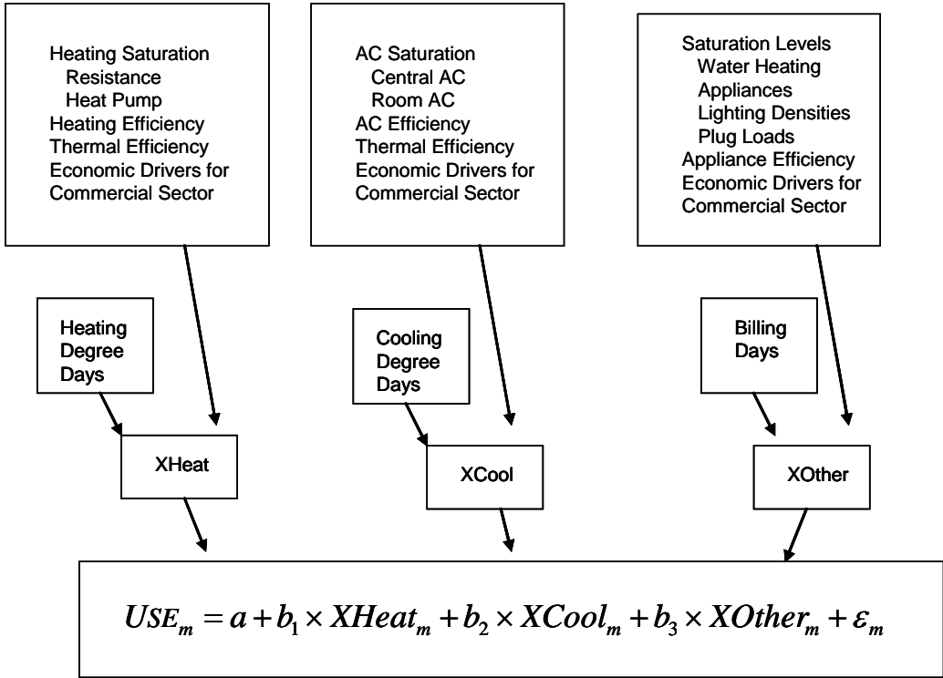
Figure A1.1 Statistically Adjusted End Use (SAE) Model
