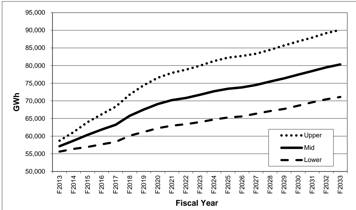
Figure 5.1 High and Low Bands for Integrated System Energy Requirements before DSM with Rate Impacts
