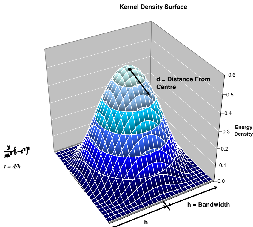
Figure C-1: Kernel Density Surface
