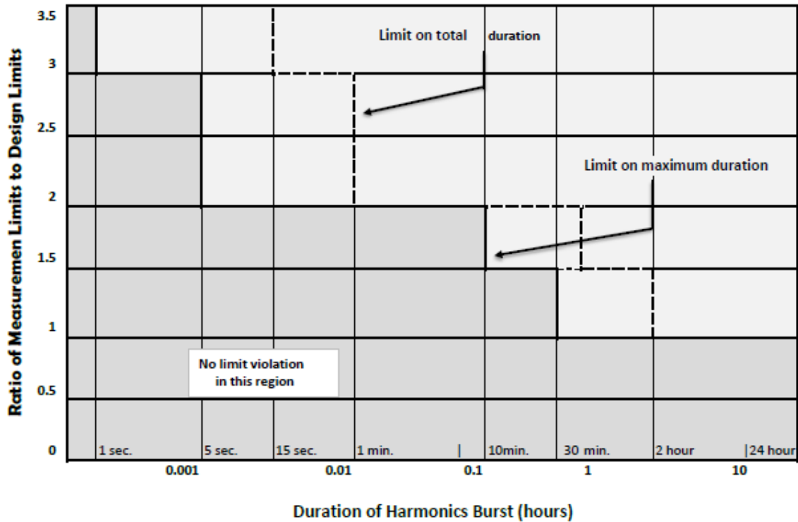
Figure 4.1: BC Hydro's Limits on measured harmonics
