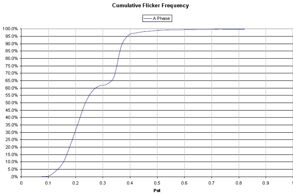
Figure 5- Voltage Flicker Accumulative flicker frequency
