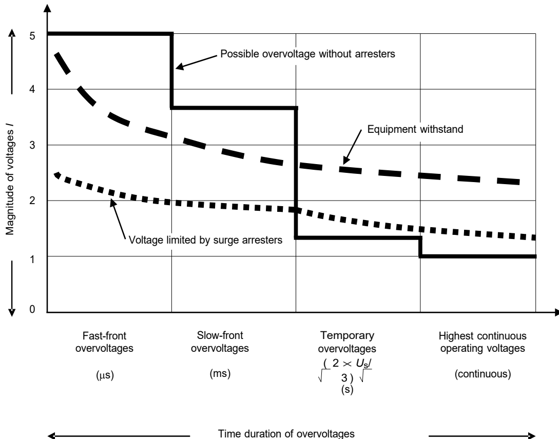
Figure C-1: Voltages and duration example for an efficiently earthed system
