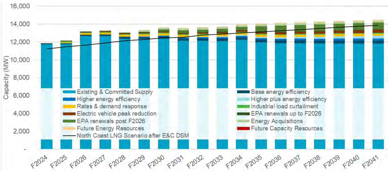
Figure 1-23 System capacity Load Resource Balance with Contingency Resource Plan for North Coast scenario
