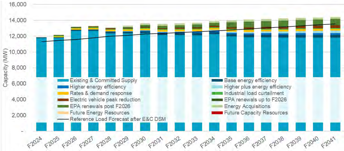
Figure 1-7 System capacity Load Resource Balance with Base Resource Plan resources
