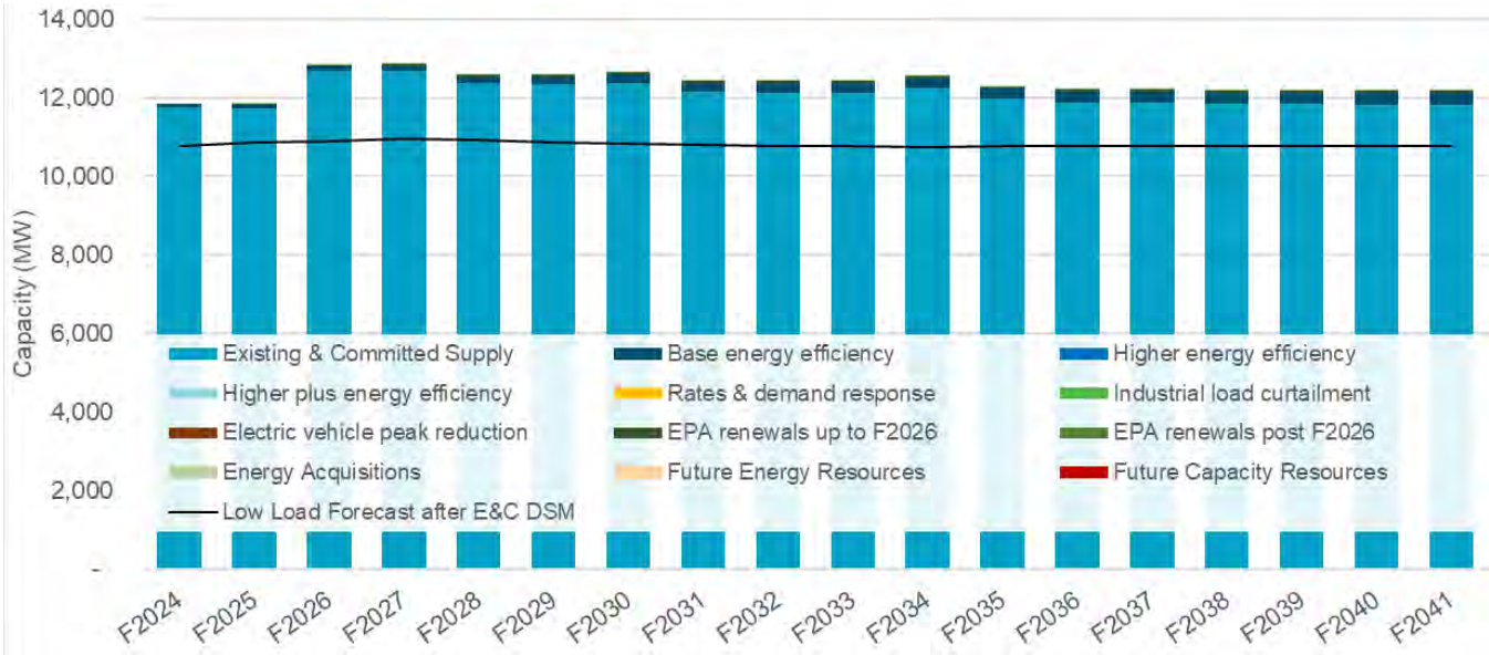
Figure 1-19 System capacity Load Resource Balance with Contingency Resource Plan for Low load scenario
