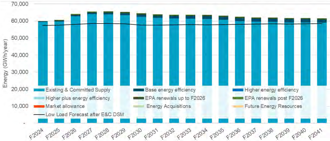
Figure 1-18 System energy Load Resource Balance with Contingency Resource Plan for Low load scenario
