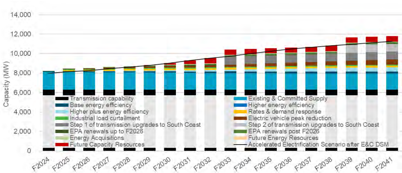
Figure 1-12 South Coast capacity Load Resource Balance with Contingency Resource Plan for Accelerated electrification scenario
