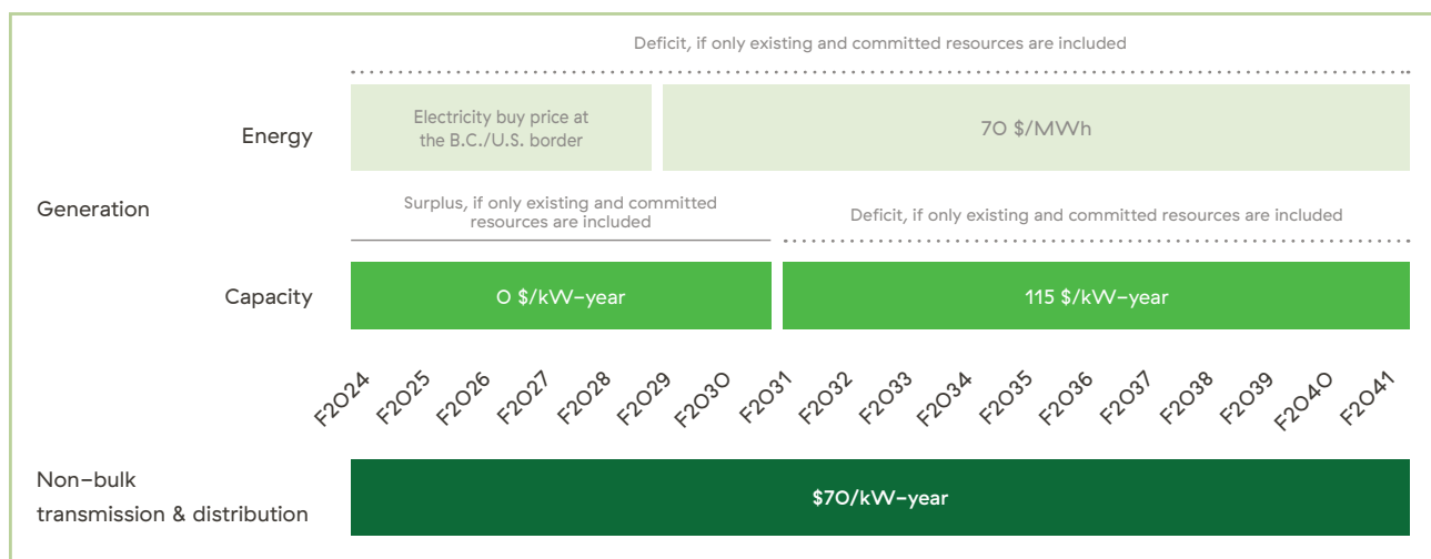
Figure 2 Reference Prices (Fiscal 2022$) Without Planned DSM and EPA Renewals Included – Updated 2021 IRP
